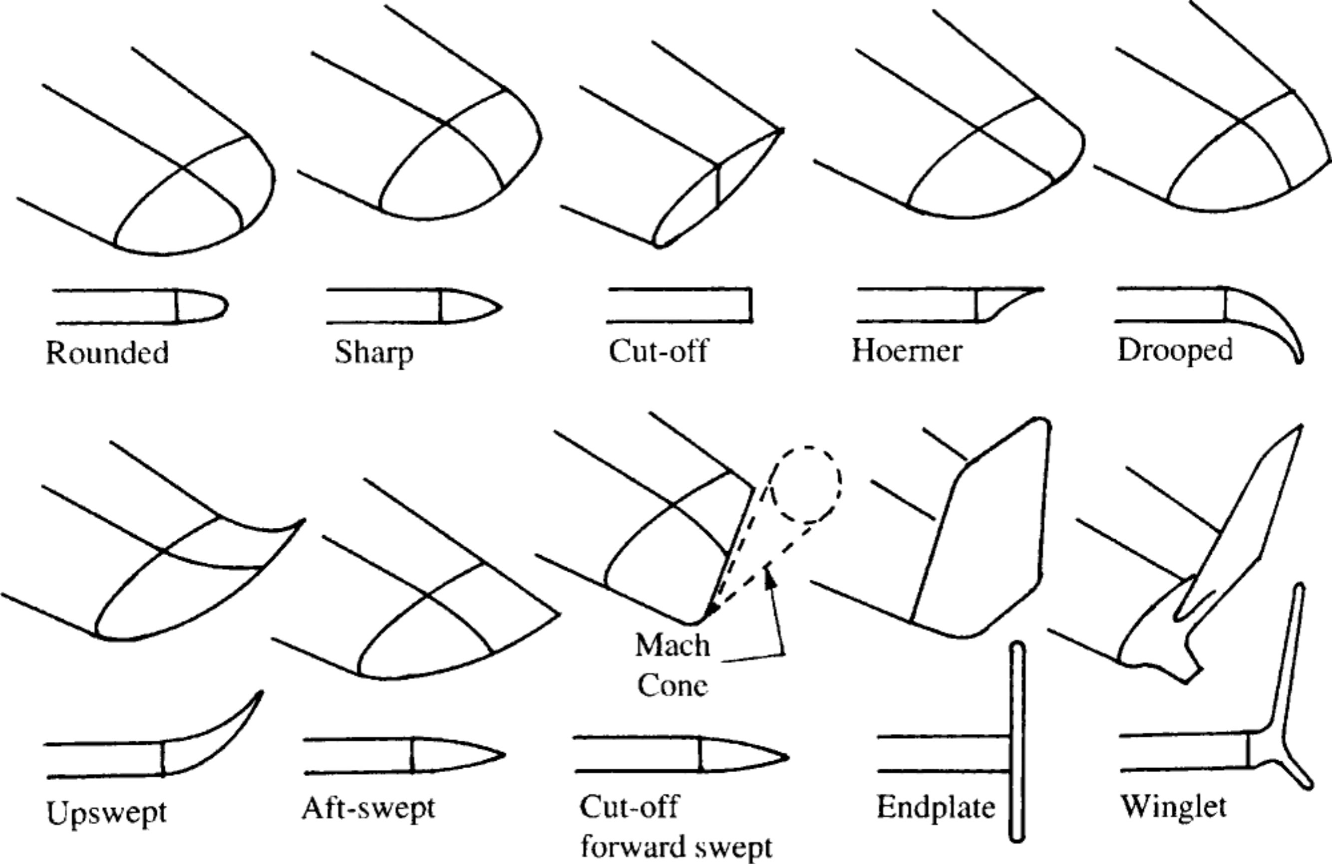
Fig. 4.29 Wing tips.
