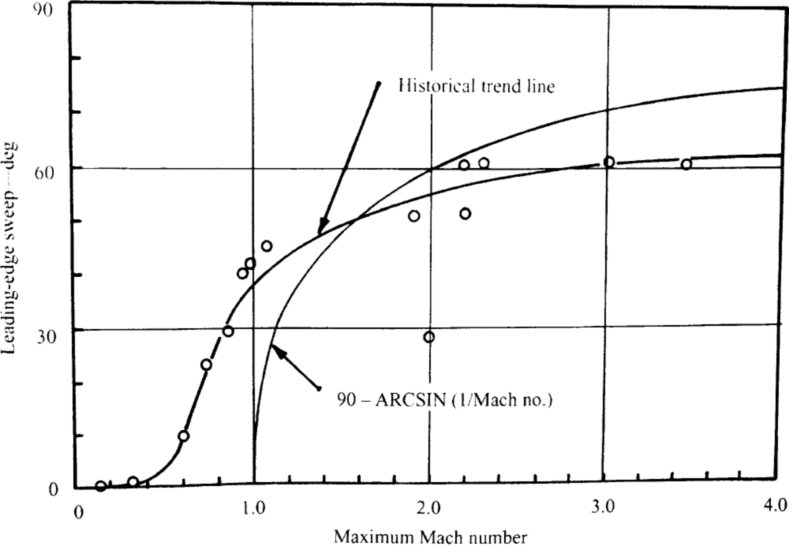
Fig. 4.20 Wing sweep historical trend.
