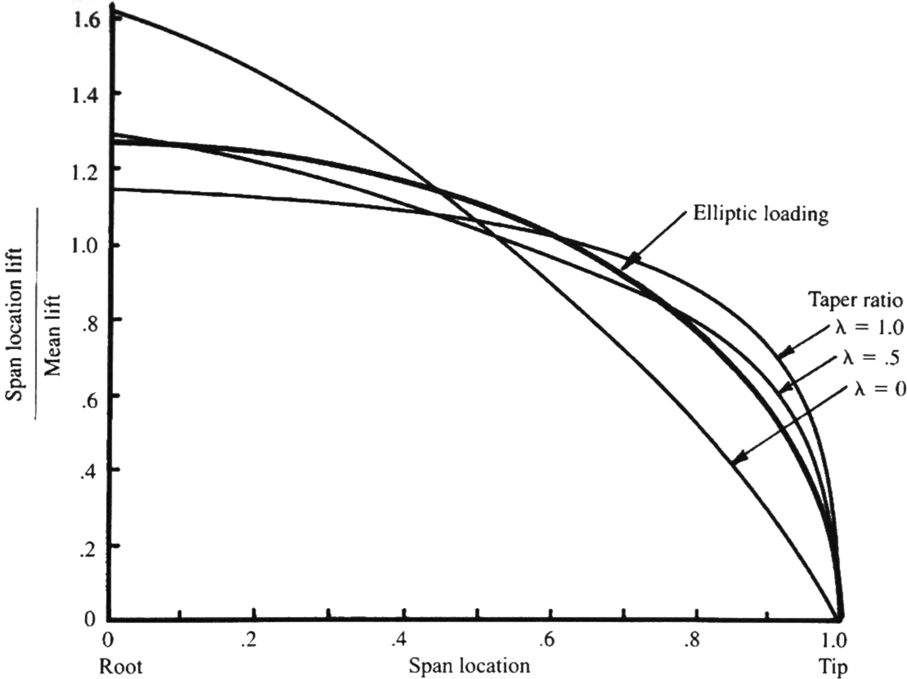
Fig. 4.23 Effect of taper on lift distribution.
