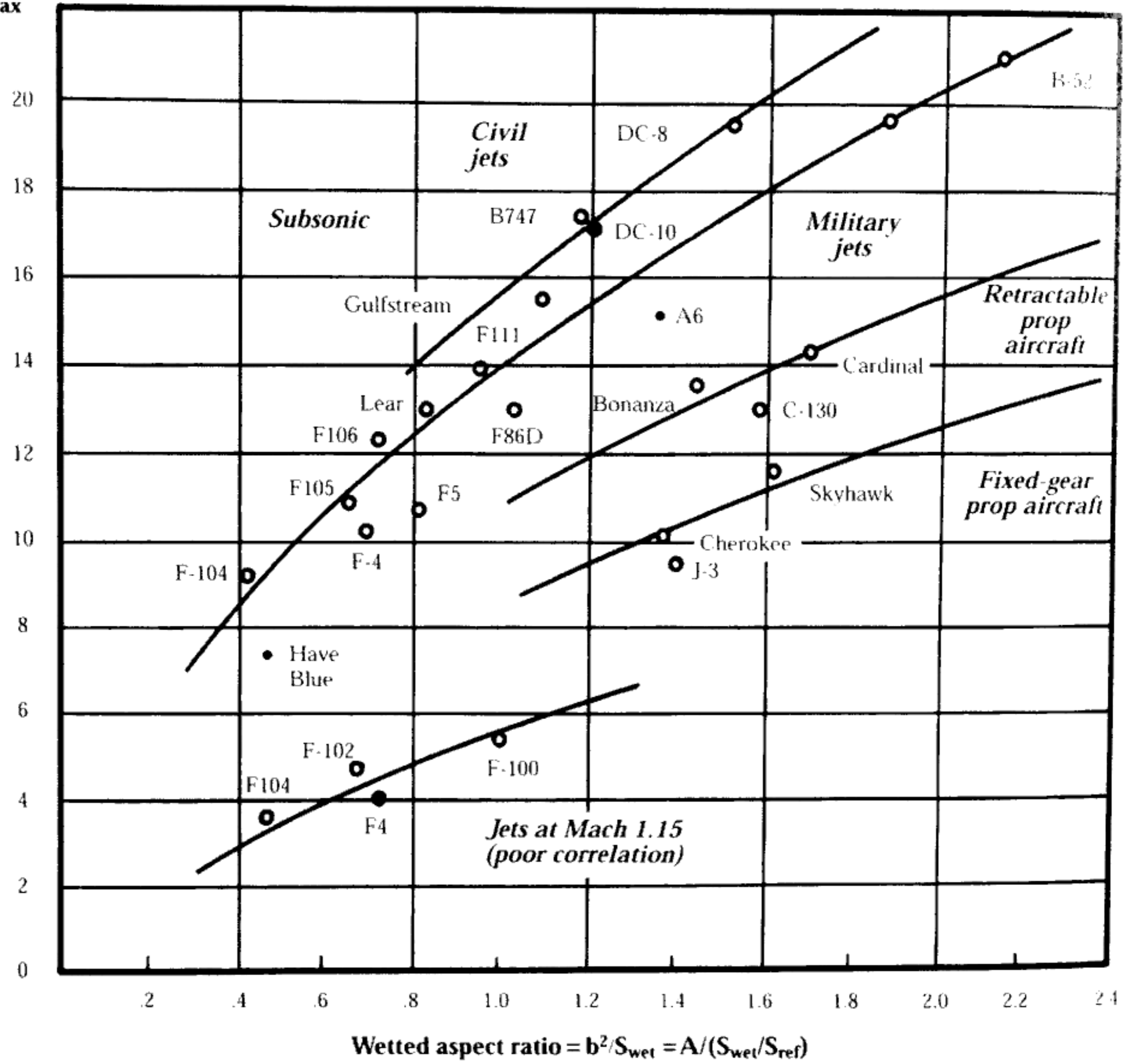
Fig. 3.6 Maximum lift-to-drag ratio trends.
