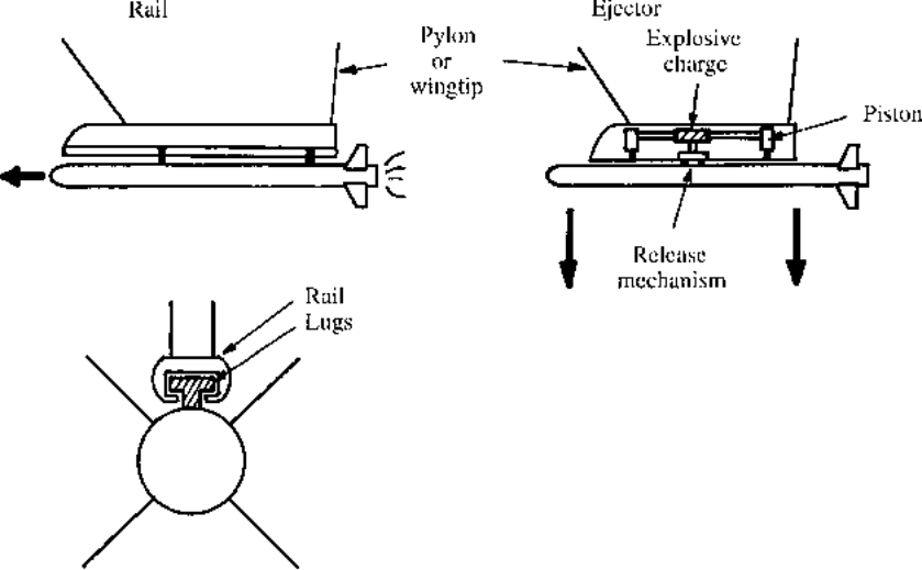
Fig. 9.5 Missile carriage/launch.
