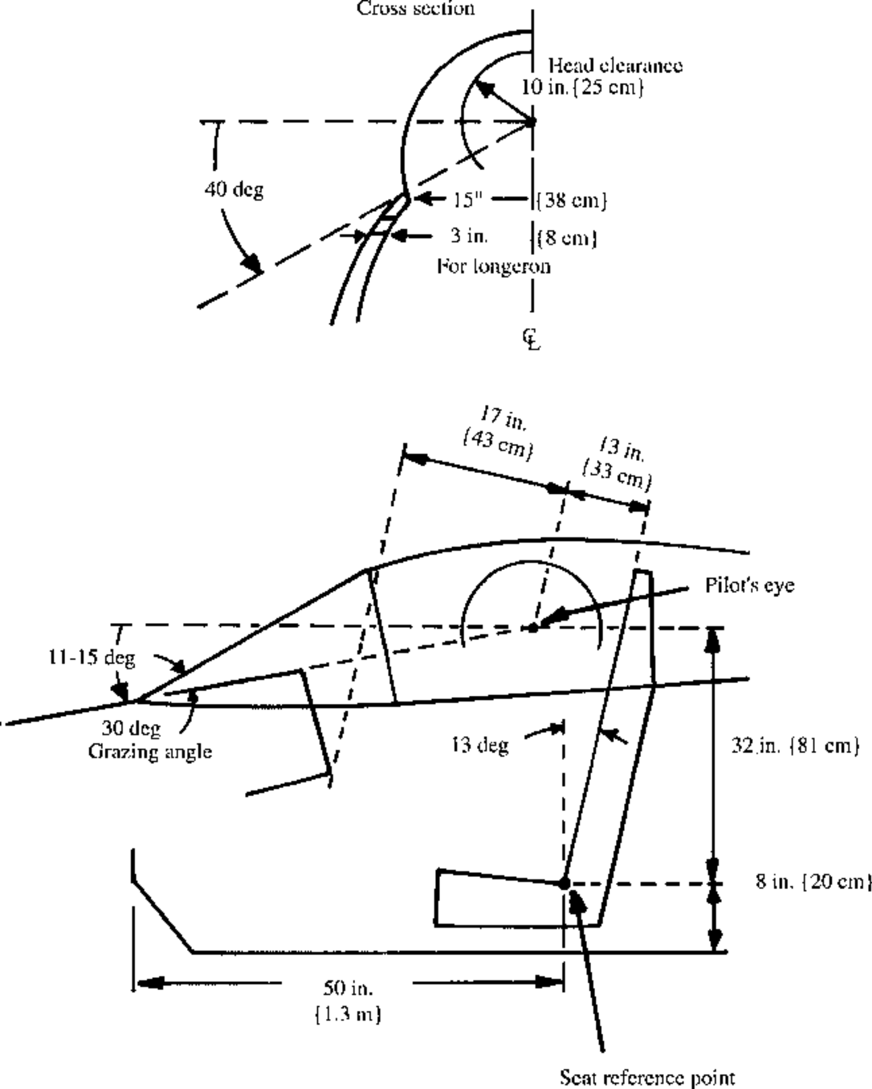
Fig. 9.2 Typical fighter cockpit.
