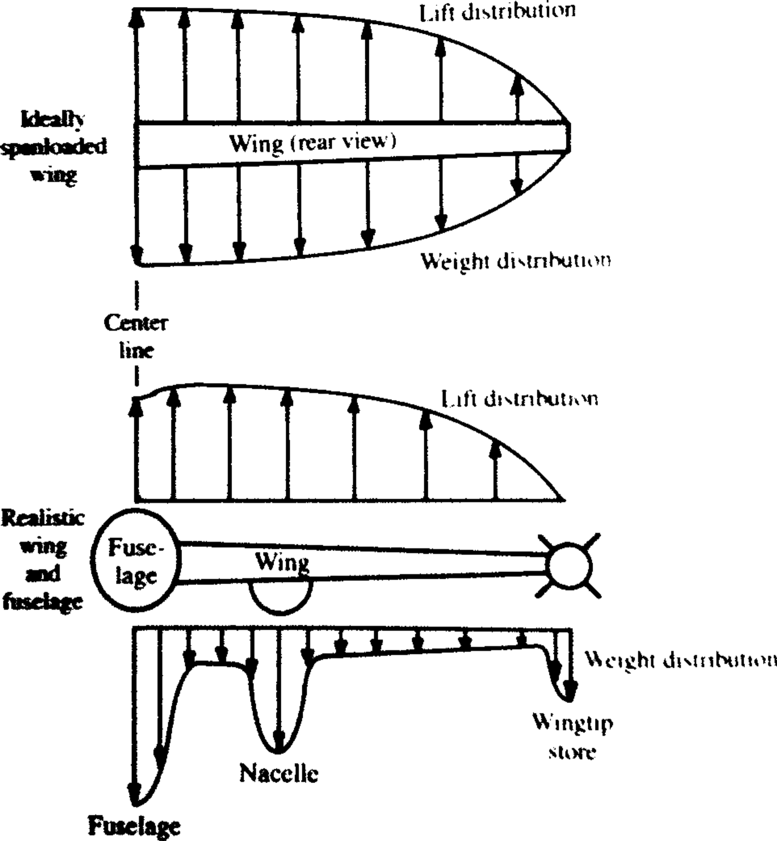
Fig. 8.8 Spanloading for weight reduction.
