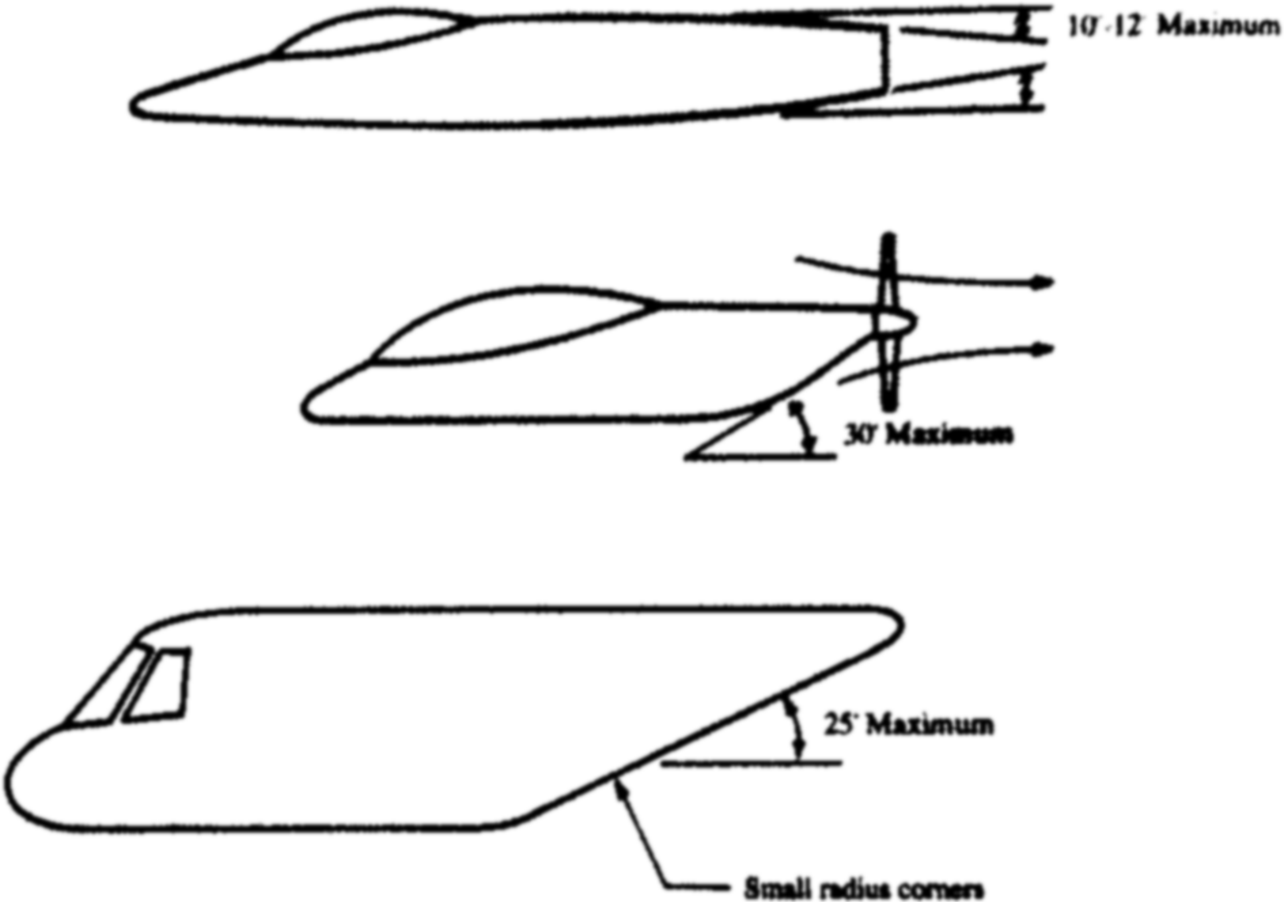
Fig. 8.1 Longitudinal contour guidelines.
