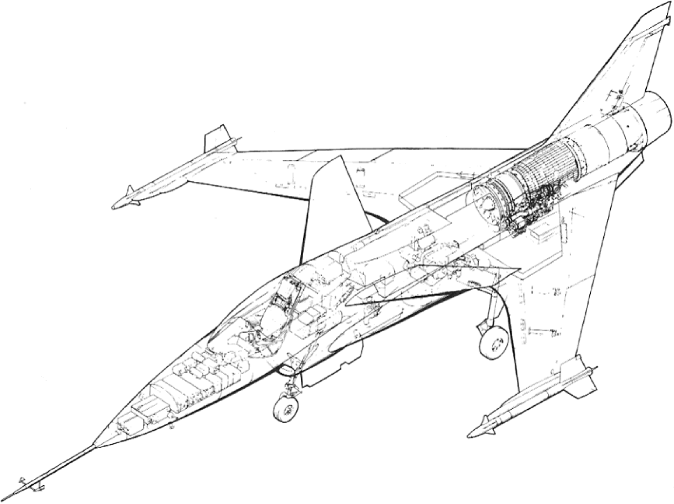
Fig. 7.8 FSW inboard isometric.
