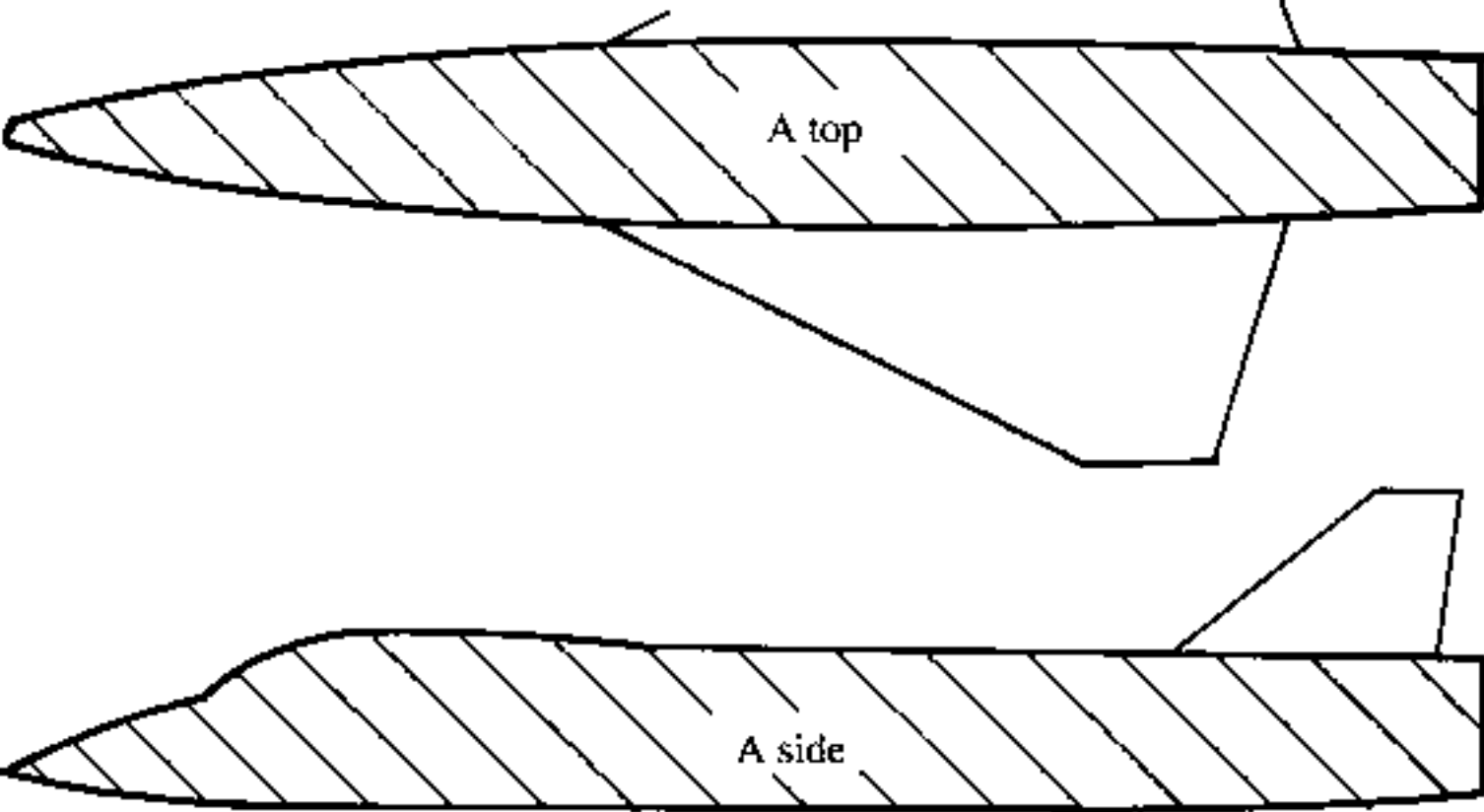
Fig. 7.36 Quick fuselage wetted area estimate.
