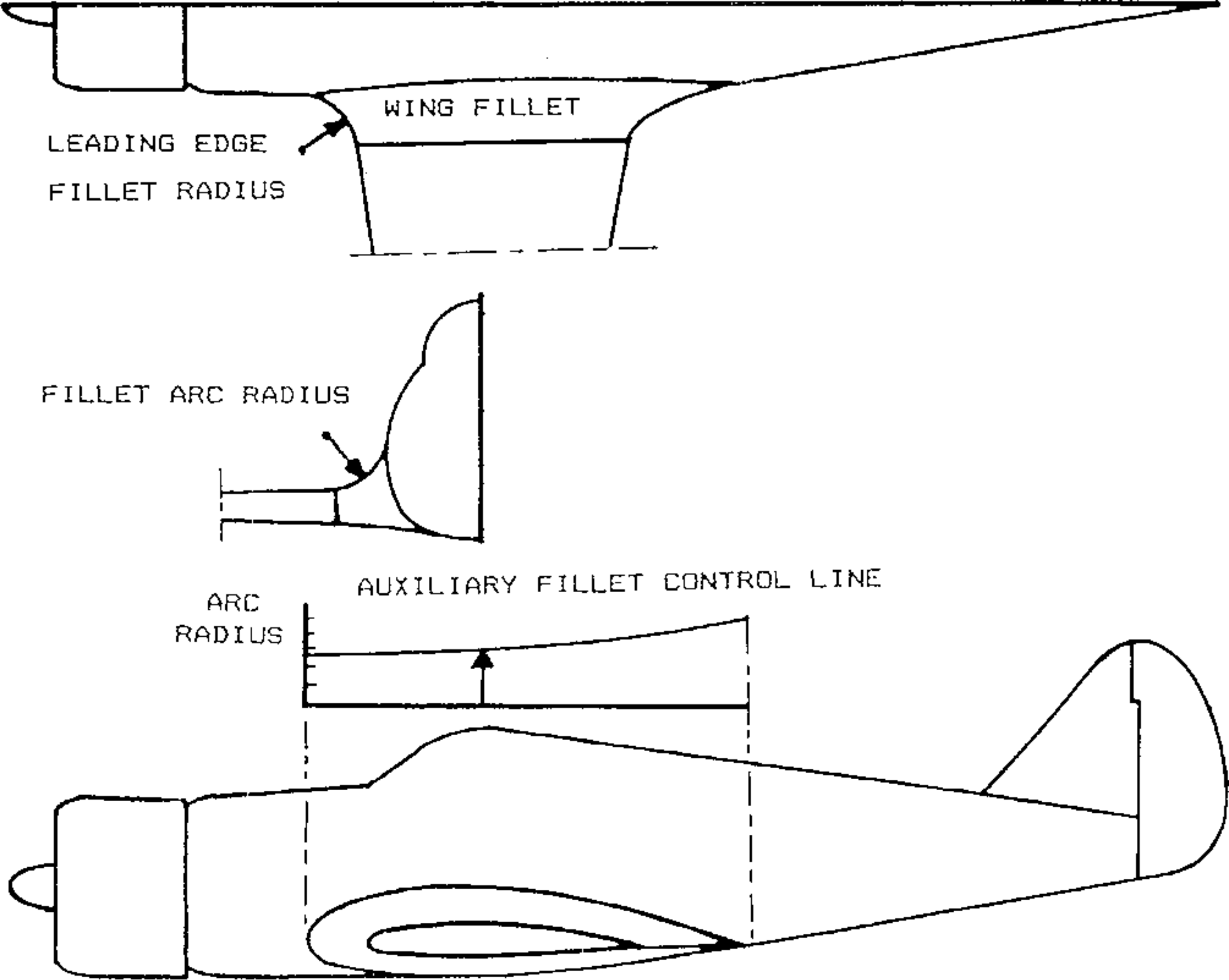
Fig. 7.33 Wing fillet layout.
