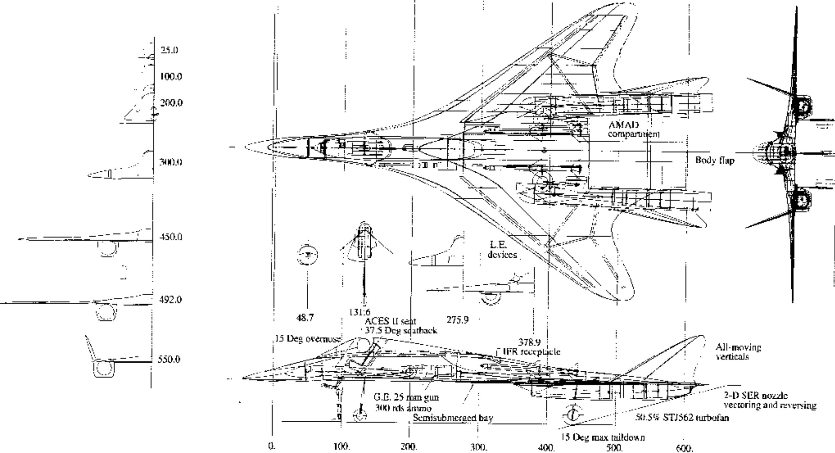
Fig. 7.3 Design layout on a CAD system.
