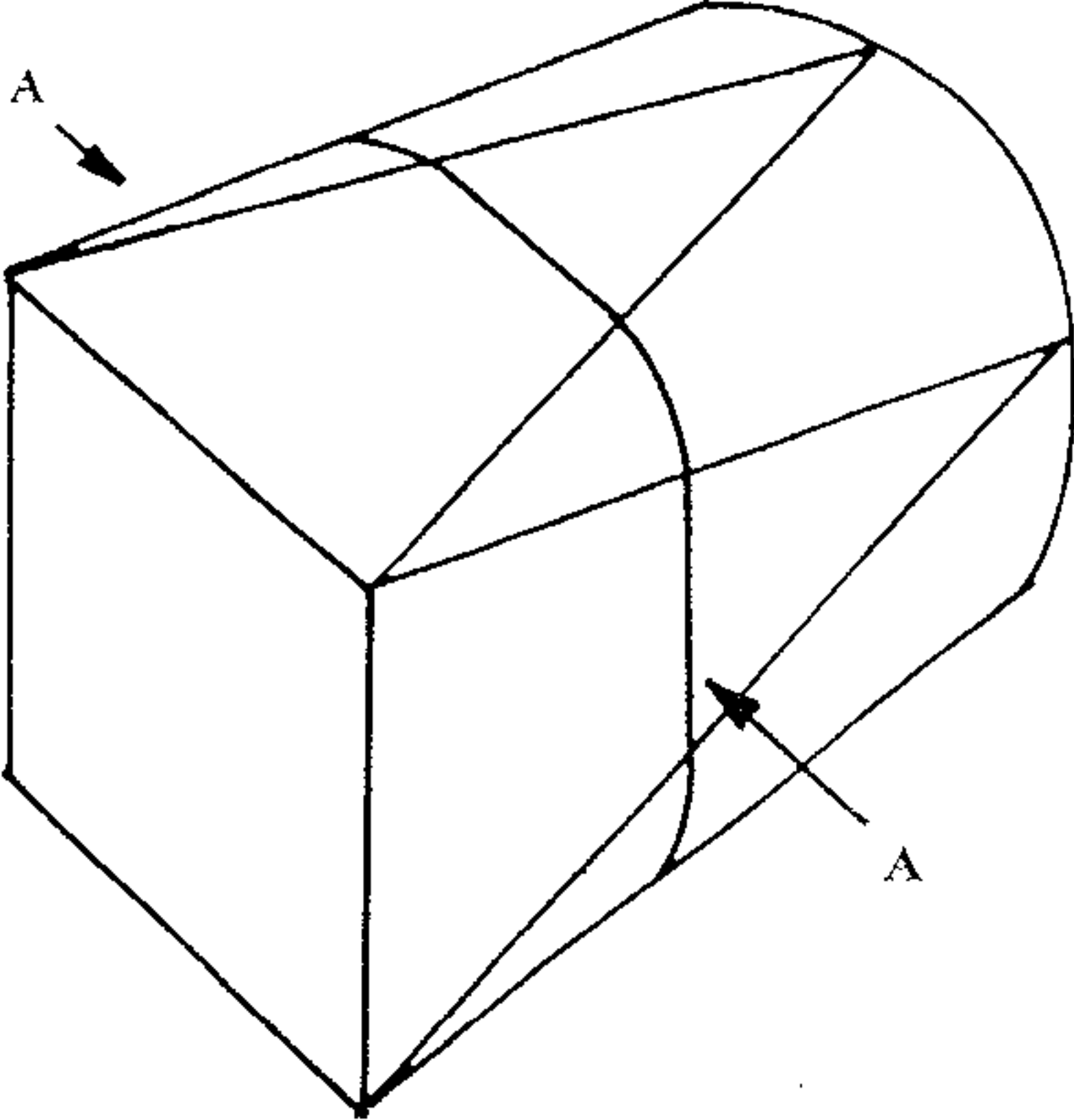
Fig. 7.20 Circle-to-square adapter.
