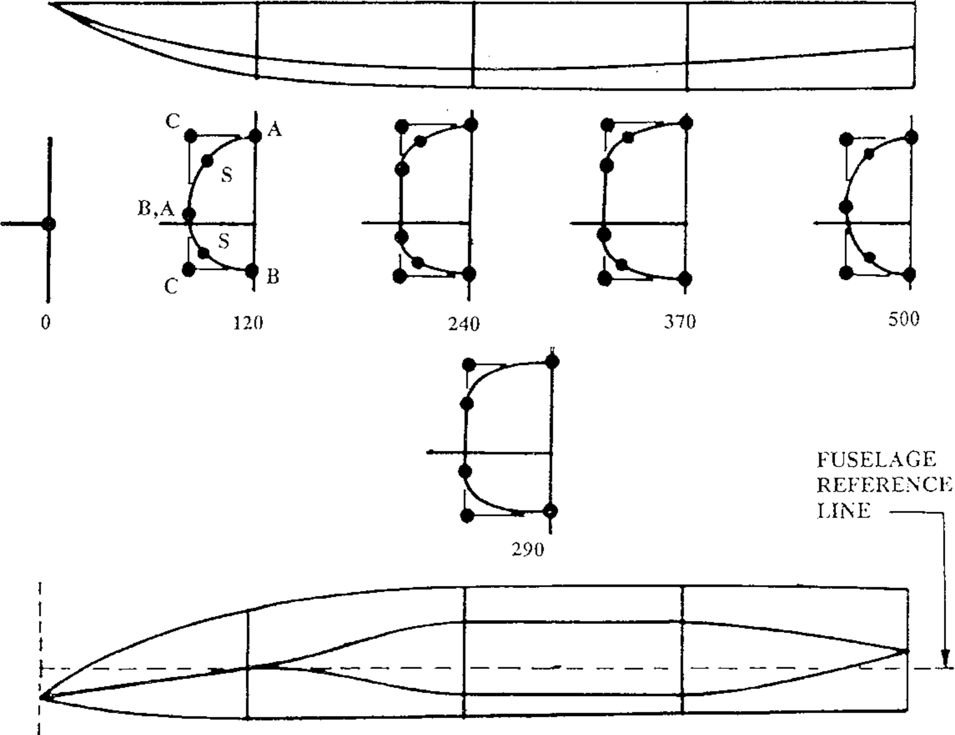
Fig. 7.15 Typical fuselage lofting.
