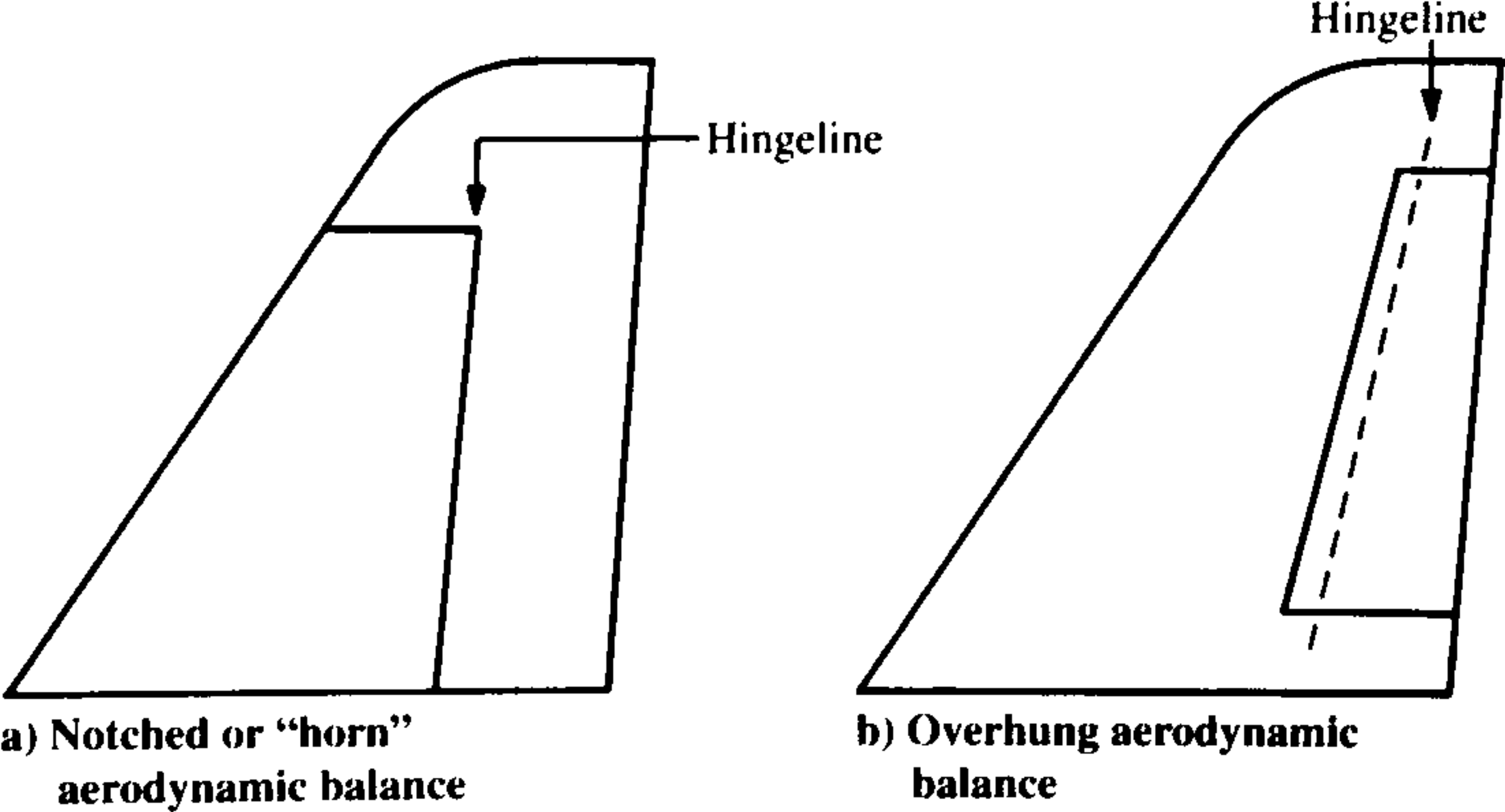
Fig. 6.5 Aerodynamic balance.
