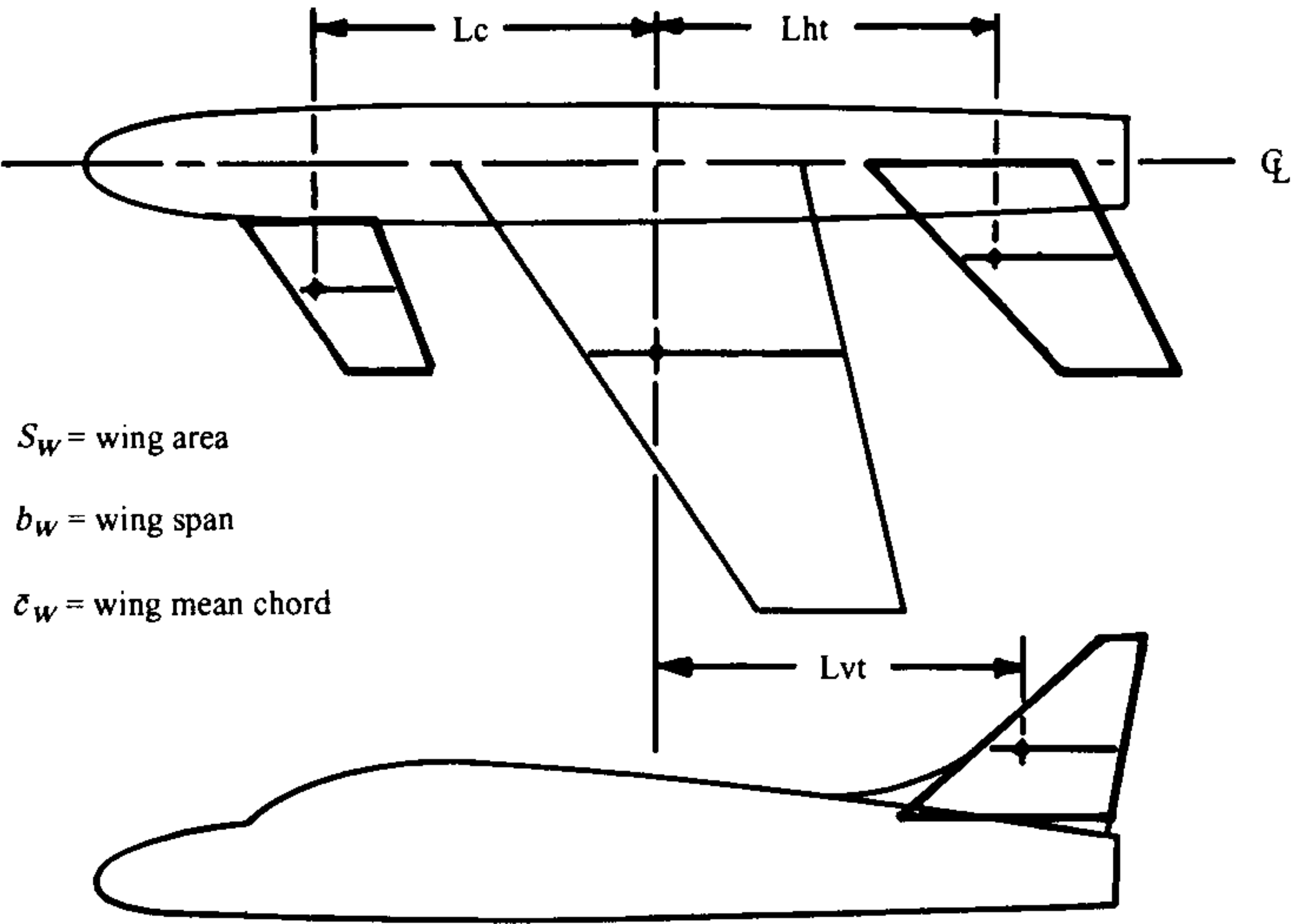
Fig. 6.2 Initial tail sizing.
