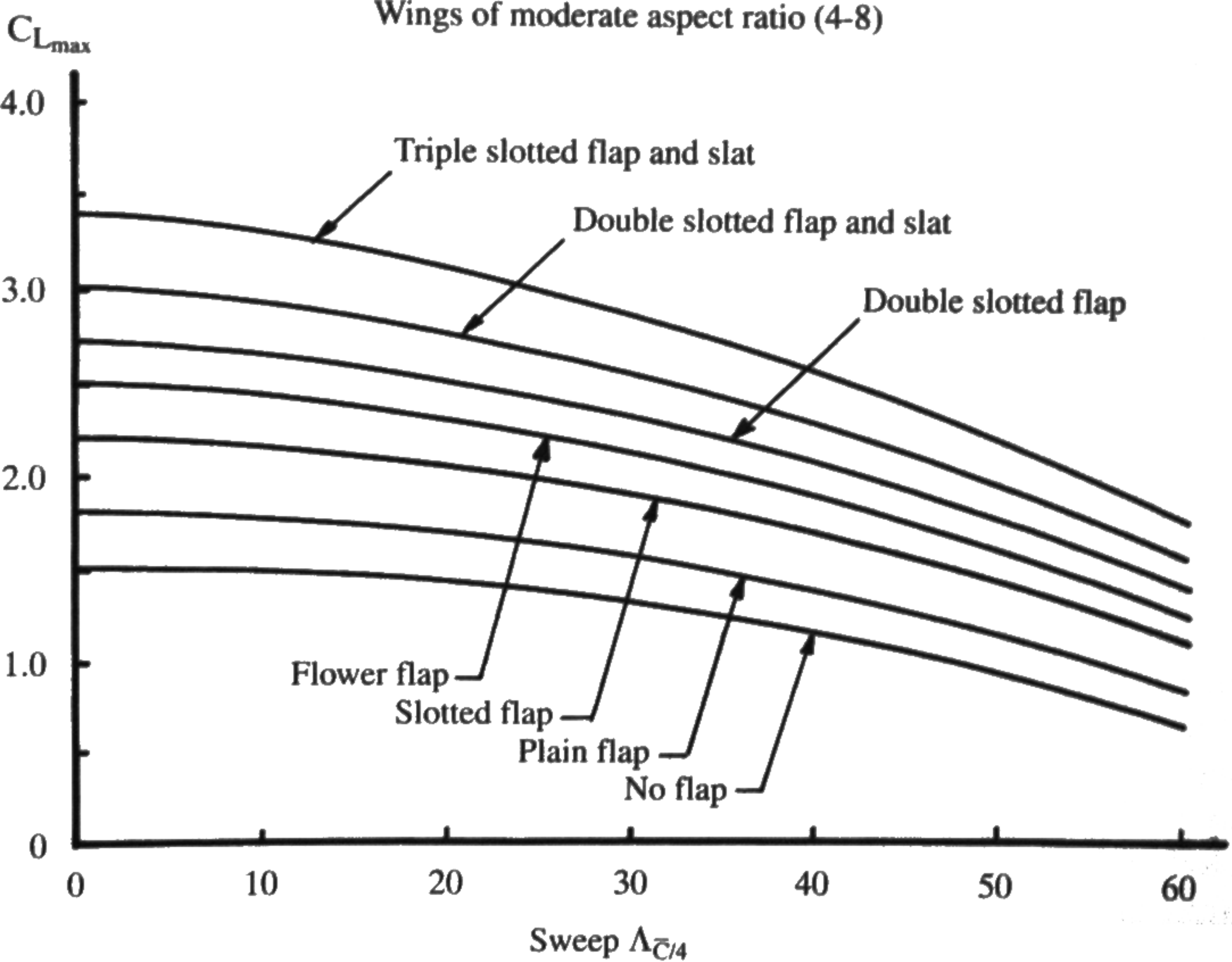
Fig. 5.3 Maximum lift coefficient.
