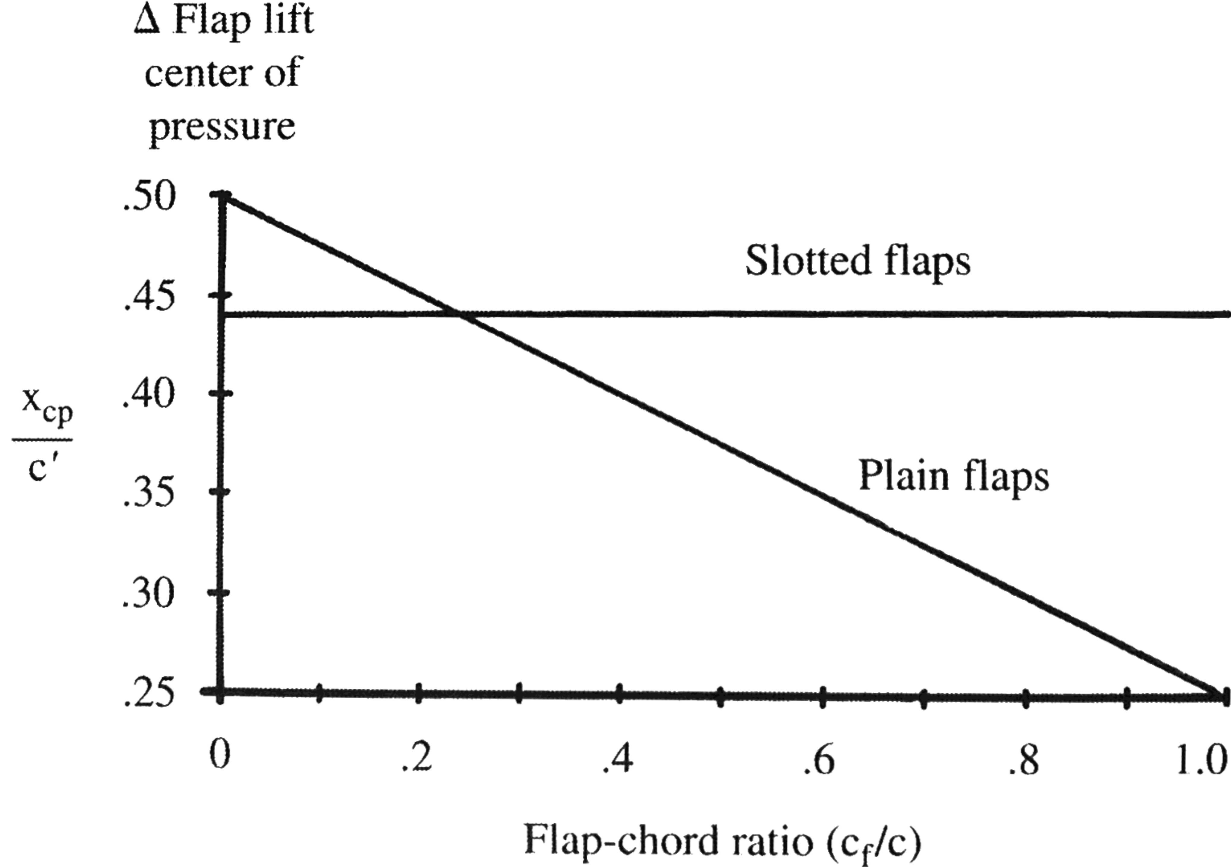
Fig. 16.9 Center of pressure for lift increment due to flaps (after Ref. 37).
