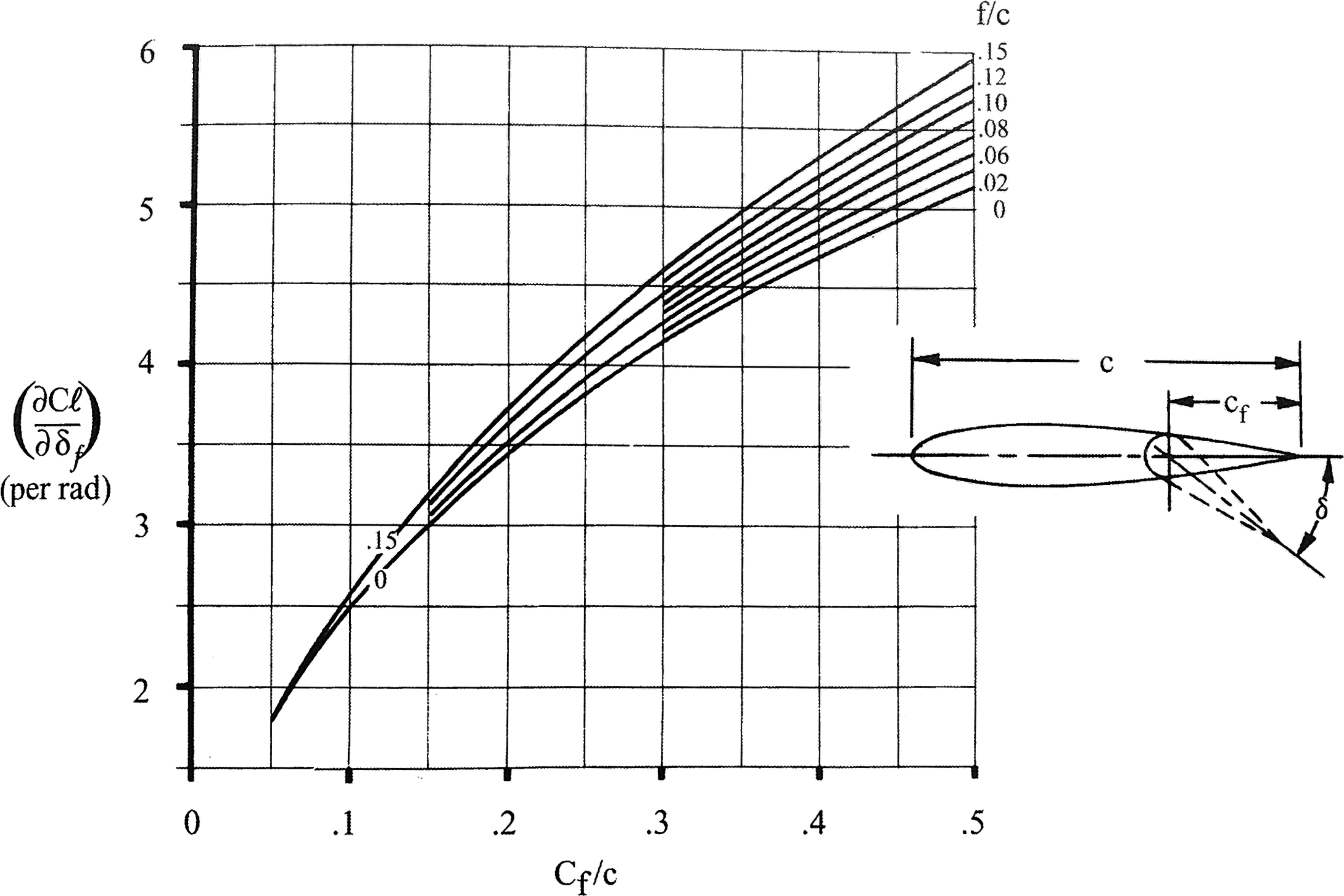
Fig. 16.6 Theoretical lift increment for plain flaps (Ref. 37).
