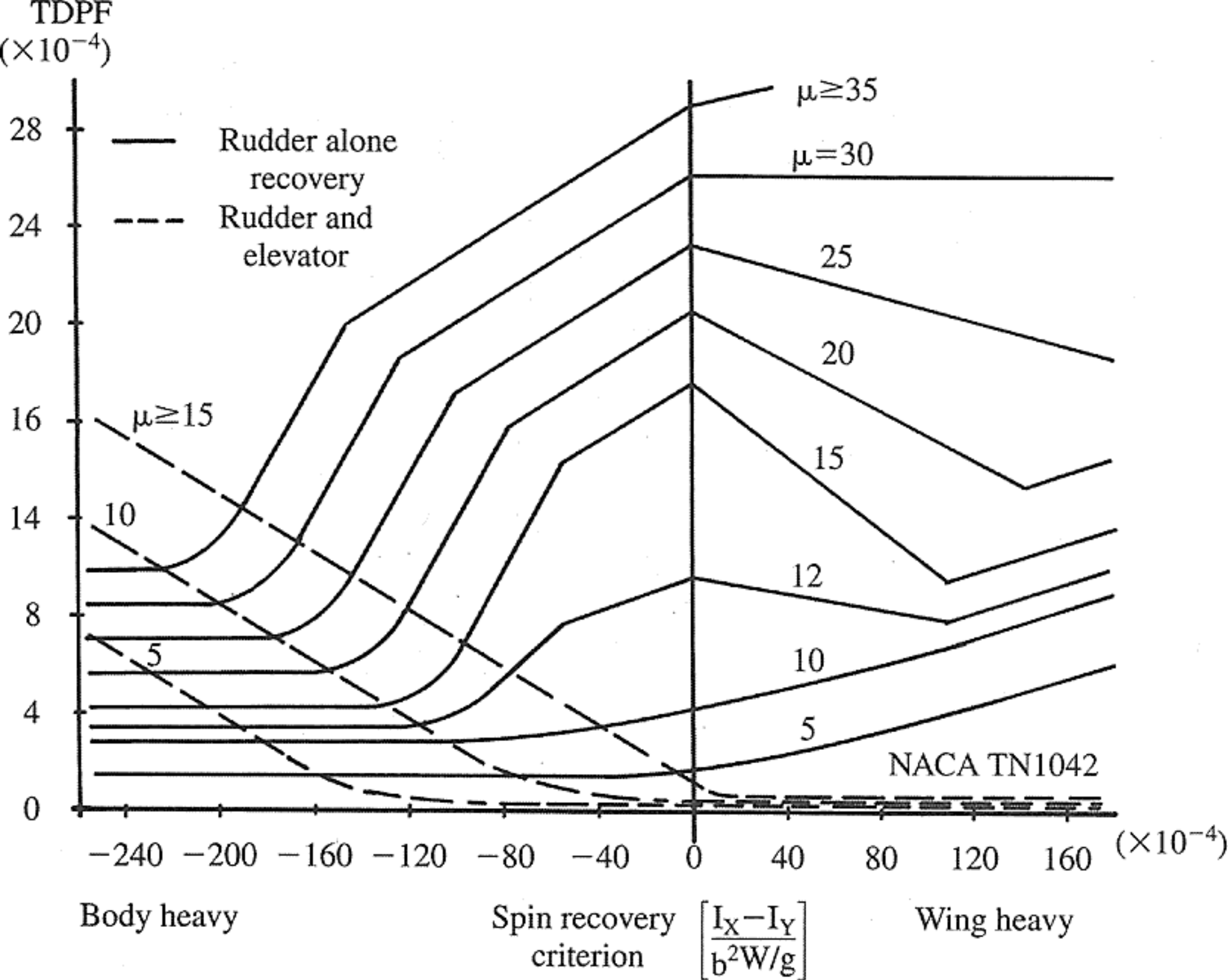
Fig. 16.32 Spin recovery criteria.
