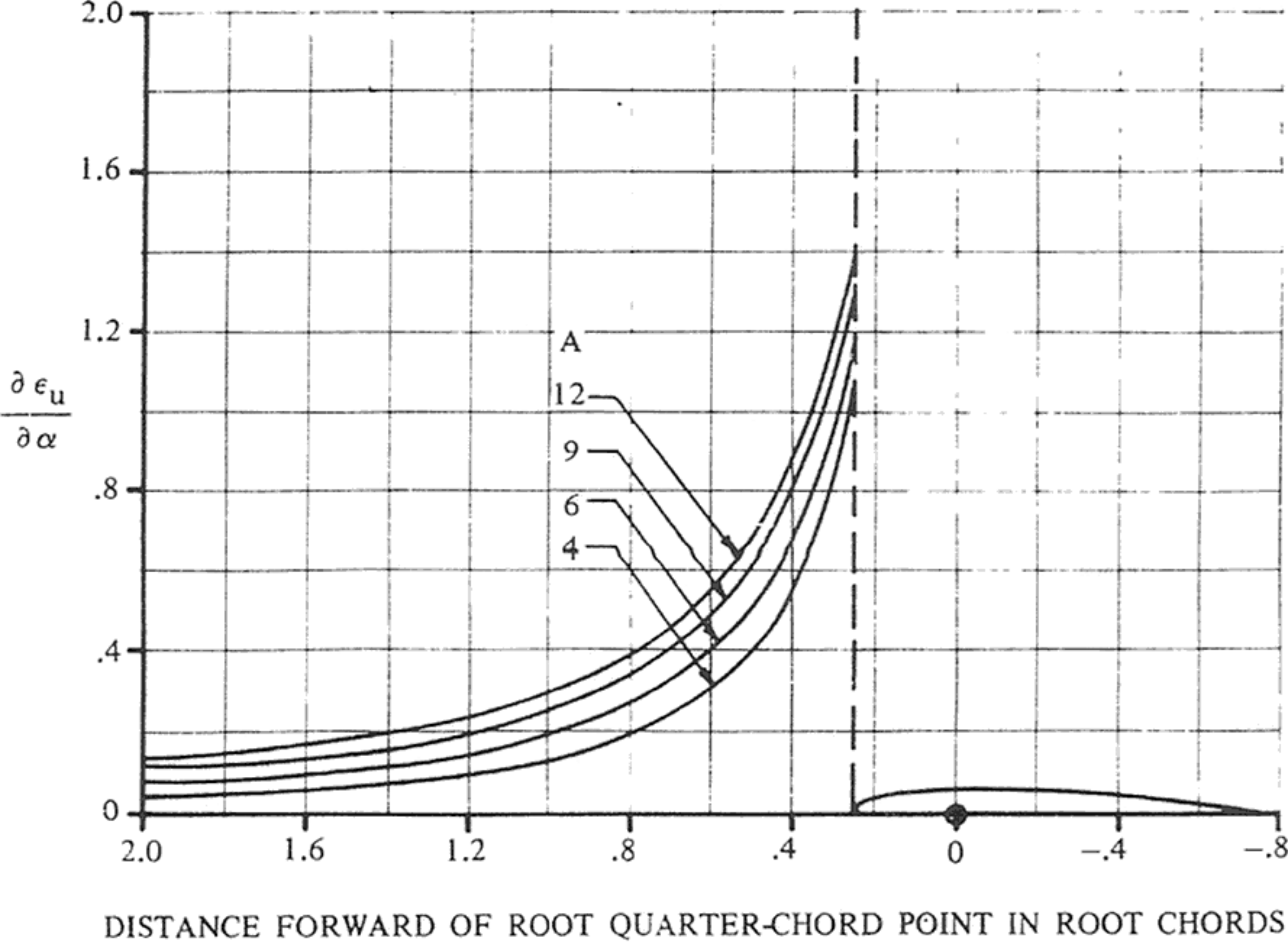
Fig. 16.11 Upwash estimation (subsonic only). (Ref. 37)
