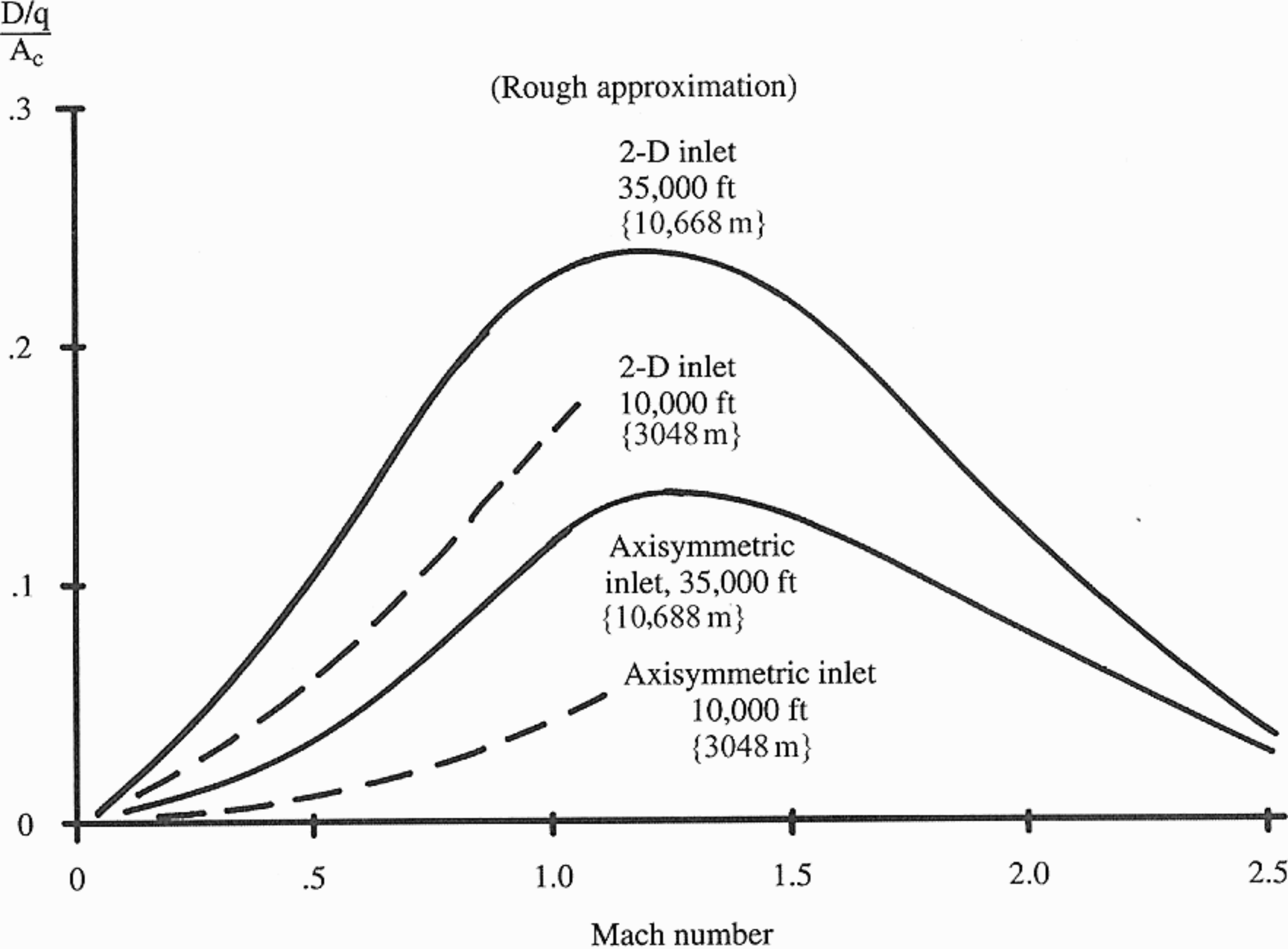
Fig. 13.9 Inlet drag trends.
