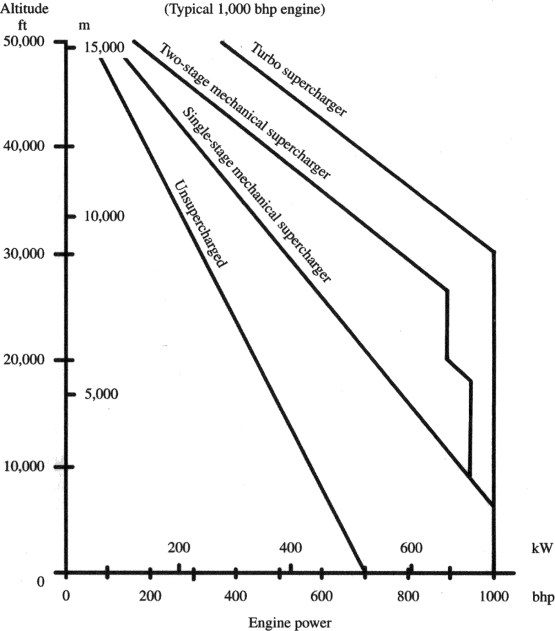
Fig. 13.10 Effects of supercharging.
