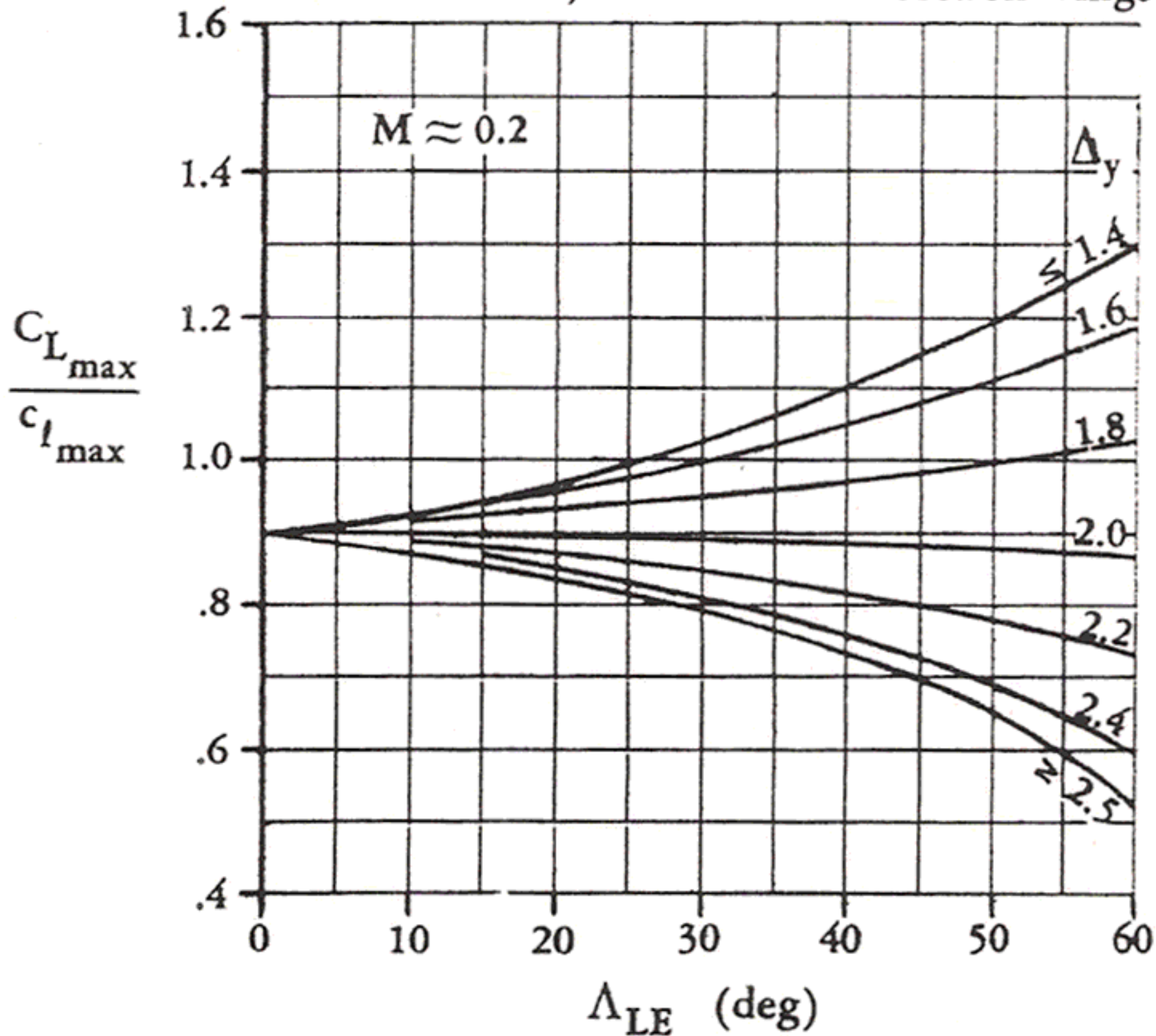
Fig. 12.8 Subsonic maximum lift of high-aspect-ratio wings. (Ref. 37)
