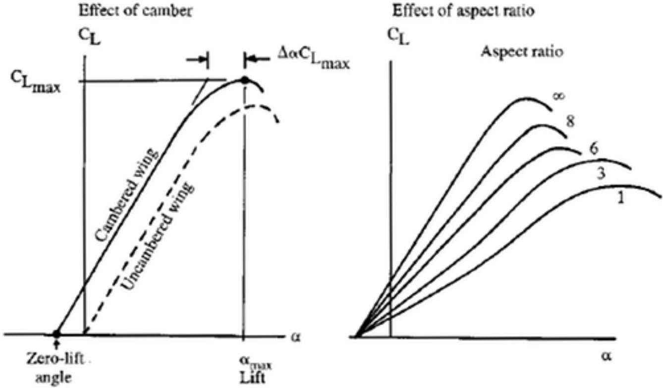
Fig. 12.4 Wing lift curve.
