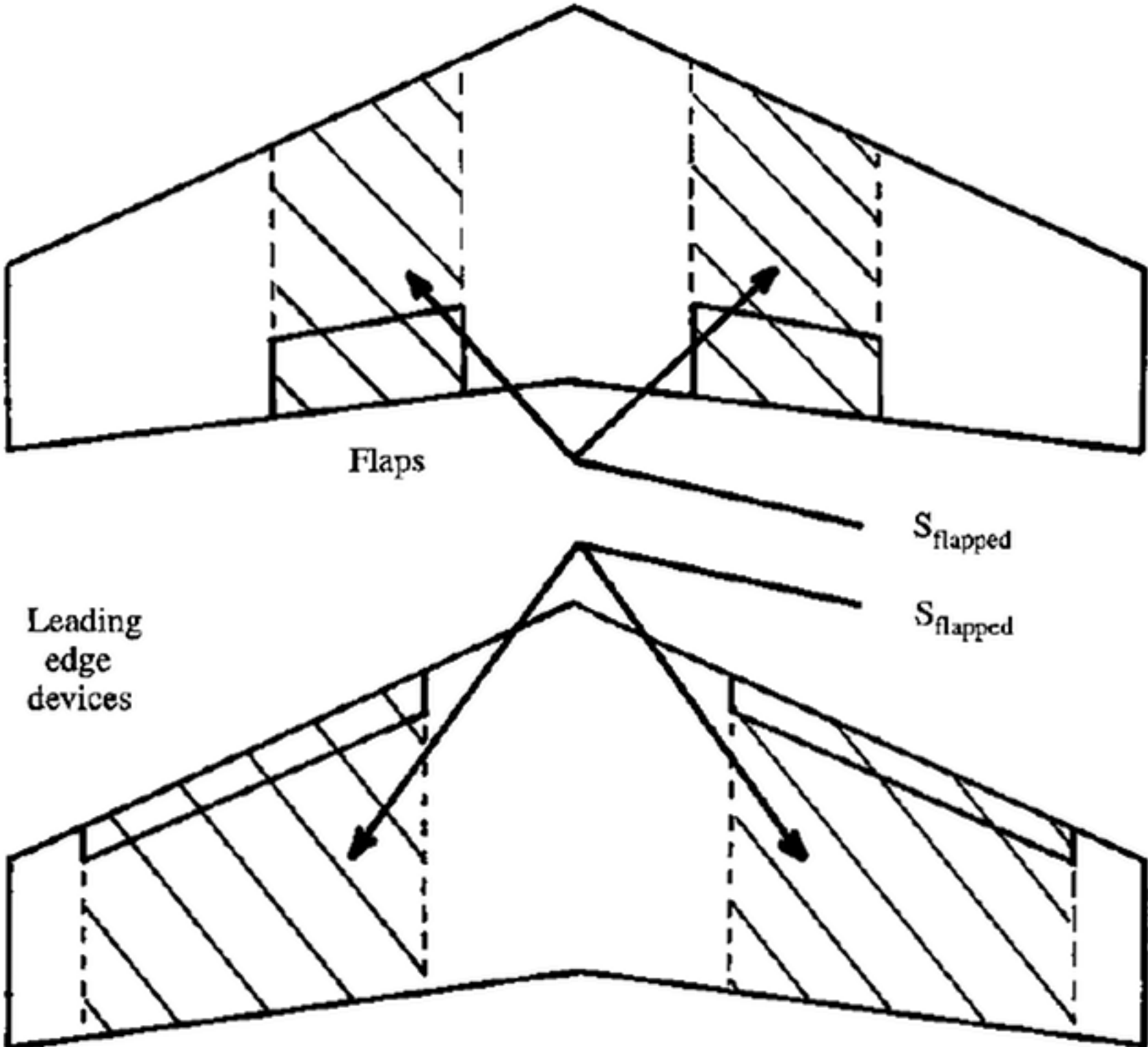
Fig. 12.20 "Flapped" wing area.
