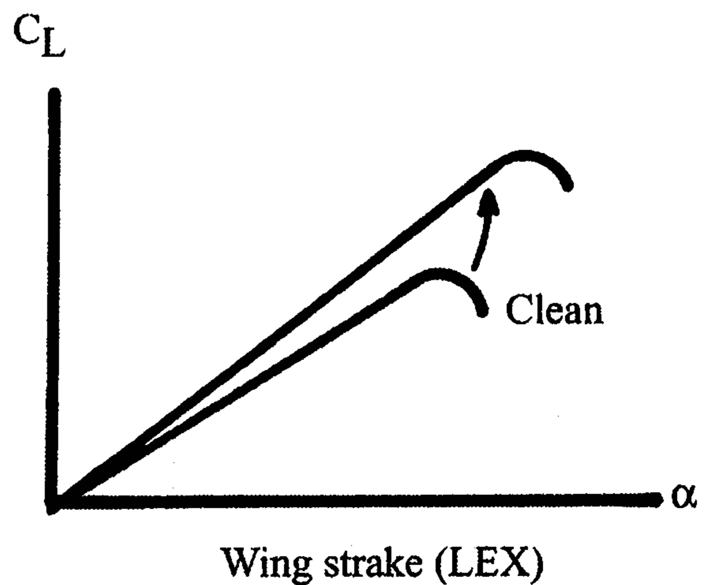
Fig. 12.19 Effects of high-lift devices.
