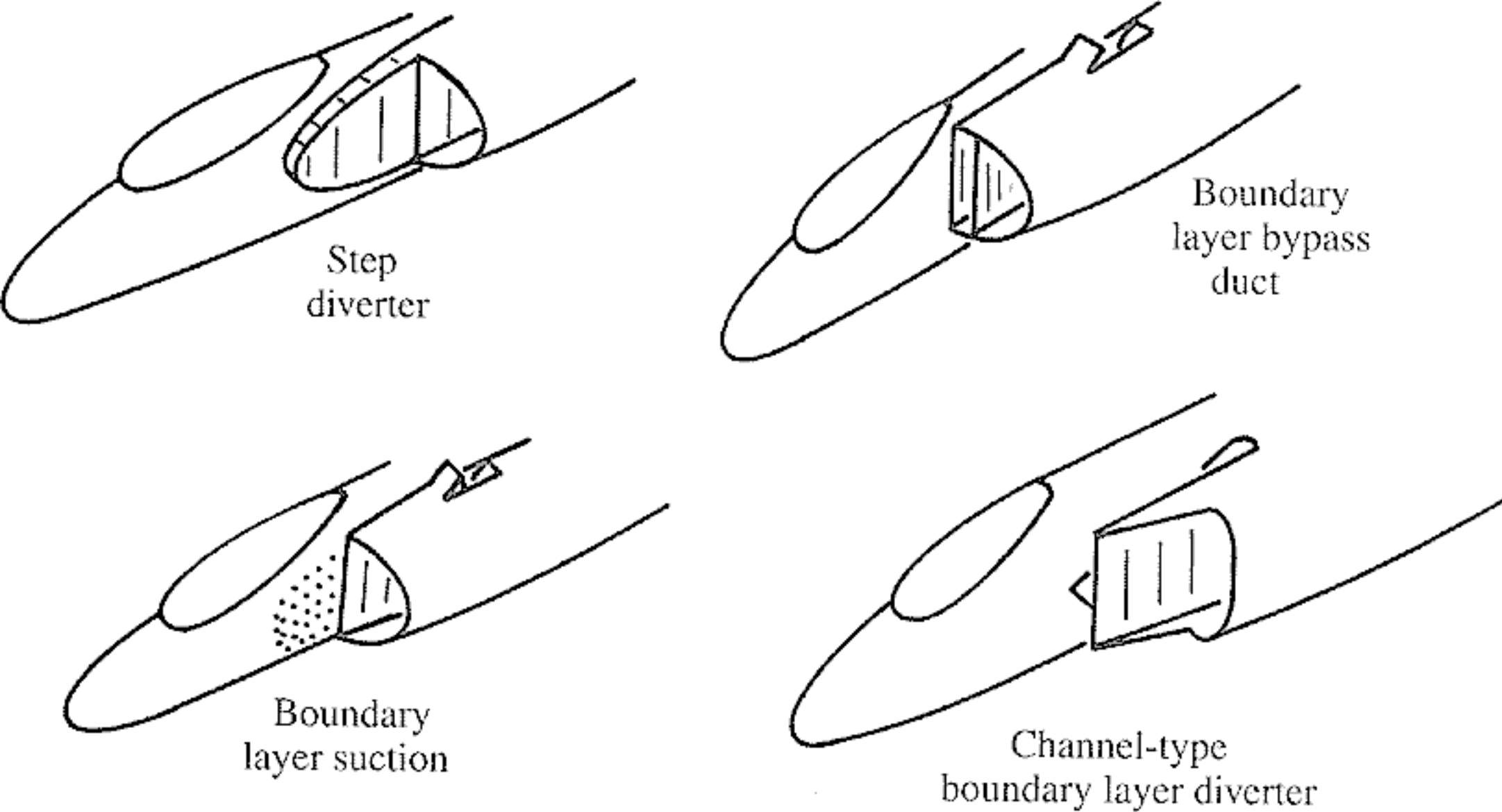
Fig. 10.21 Boundary-layer removal.
