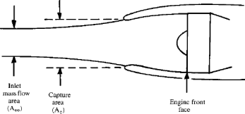
Fig. 10.17 Subsonic inlet capture area.
