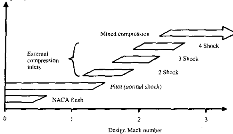
Fig. 10.13 Inlet applicability.
