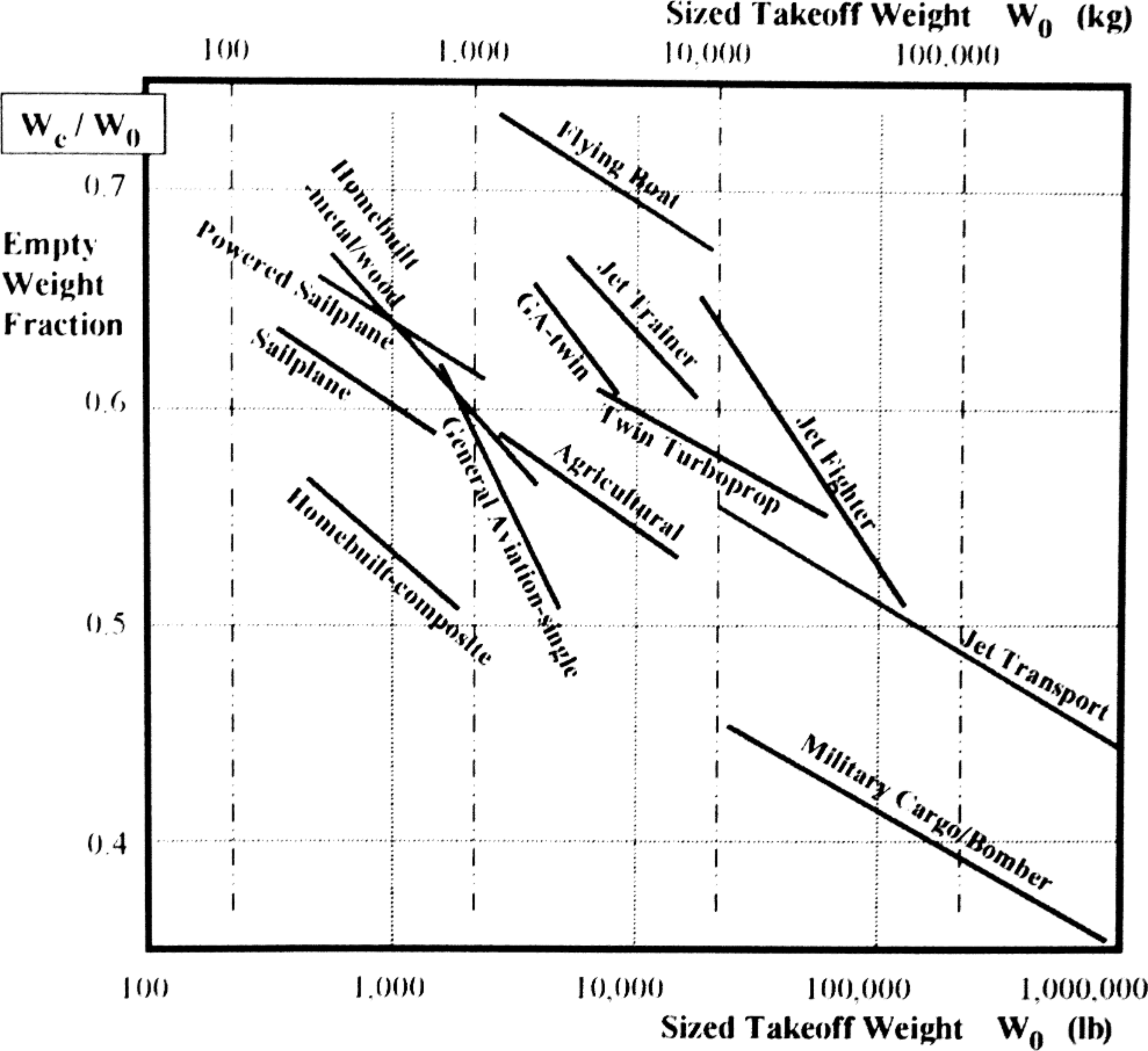
Fig. 3.1 Empty-weight fraction trends.
