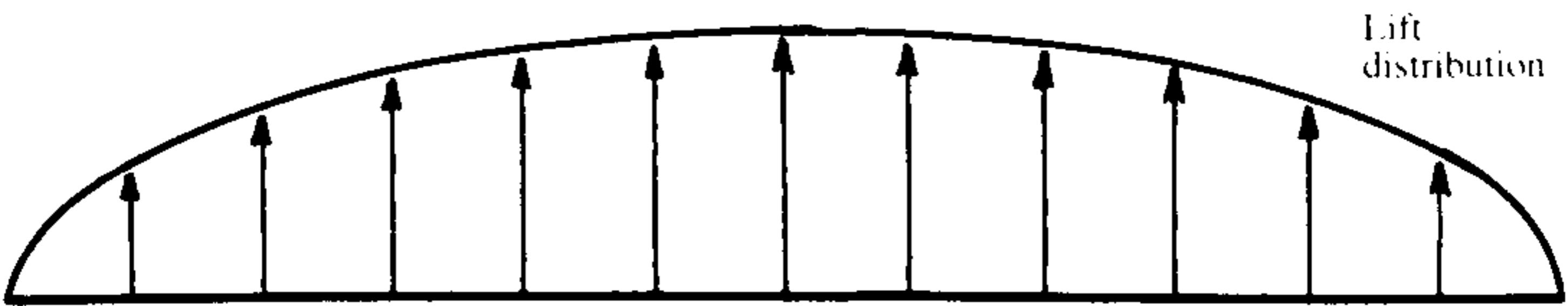
Fig. 4.22 Elliptical wing.
