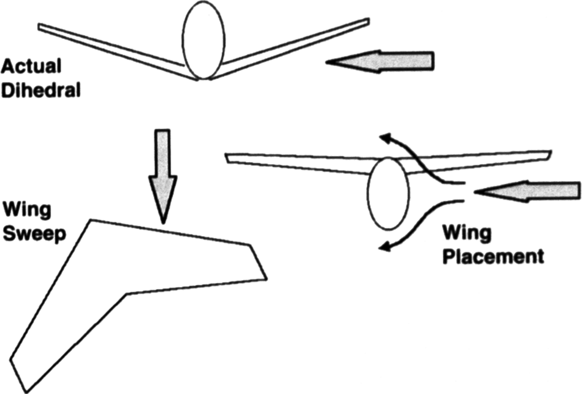
Fig. 4.25 Increased angle of attack and lift.
