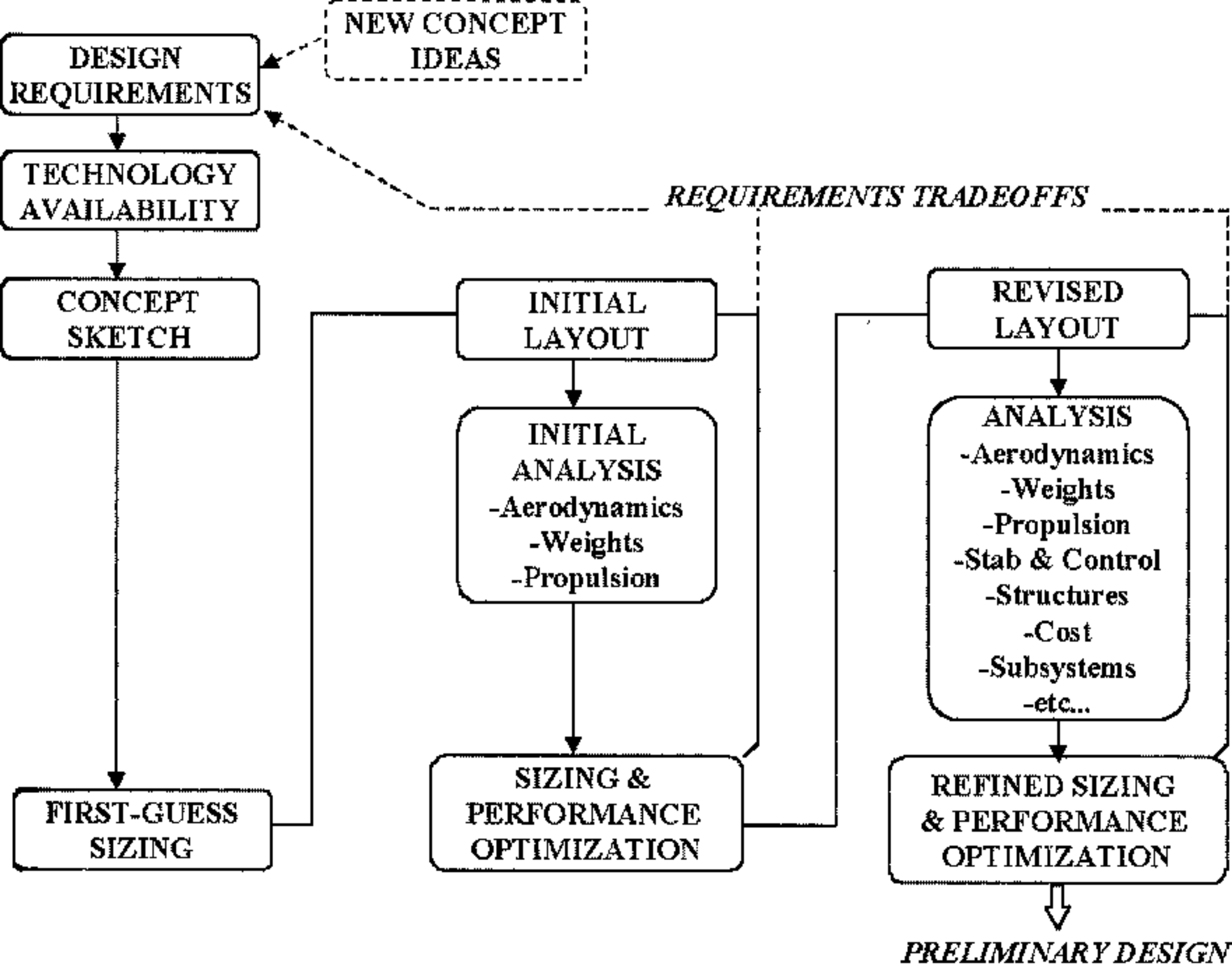
Fig. 2.4 Aircraft conceptual design process.
