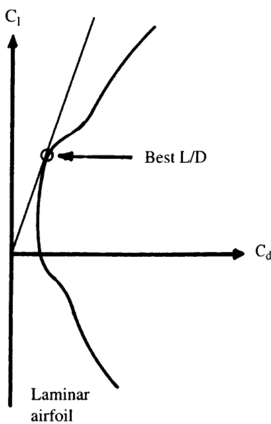
Fig. 4.9 Design lift coefficient.
