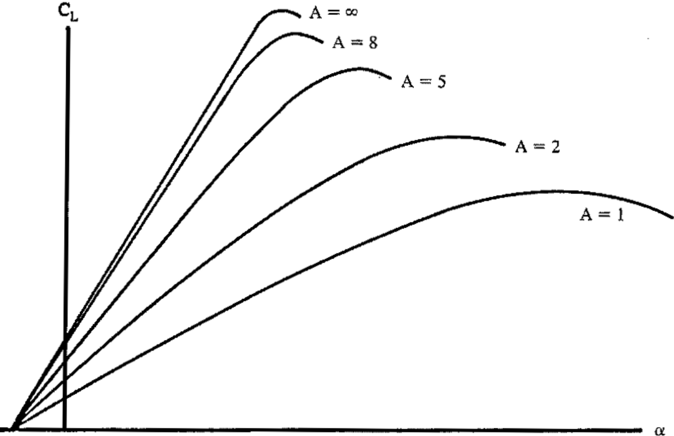
Fig. 4.19 Effect of aspect ratio on lift.
