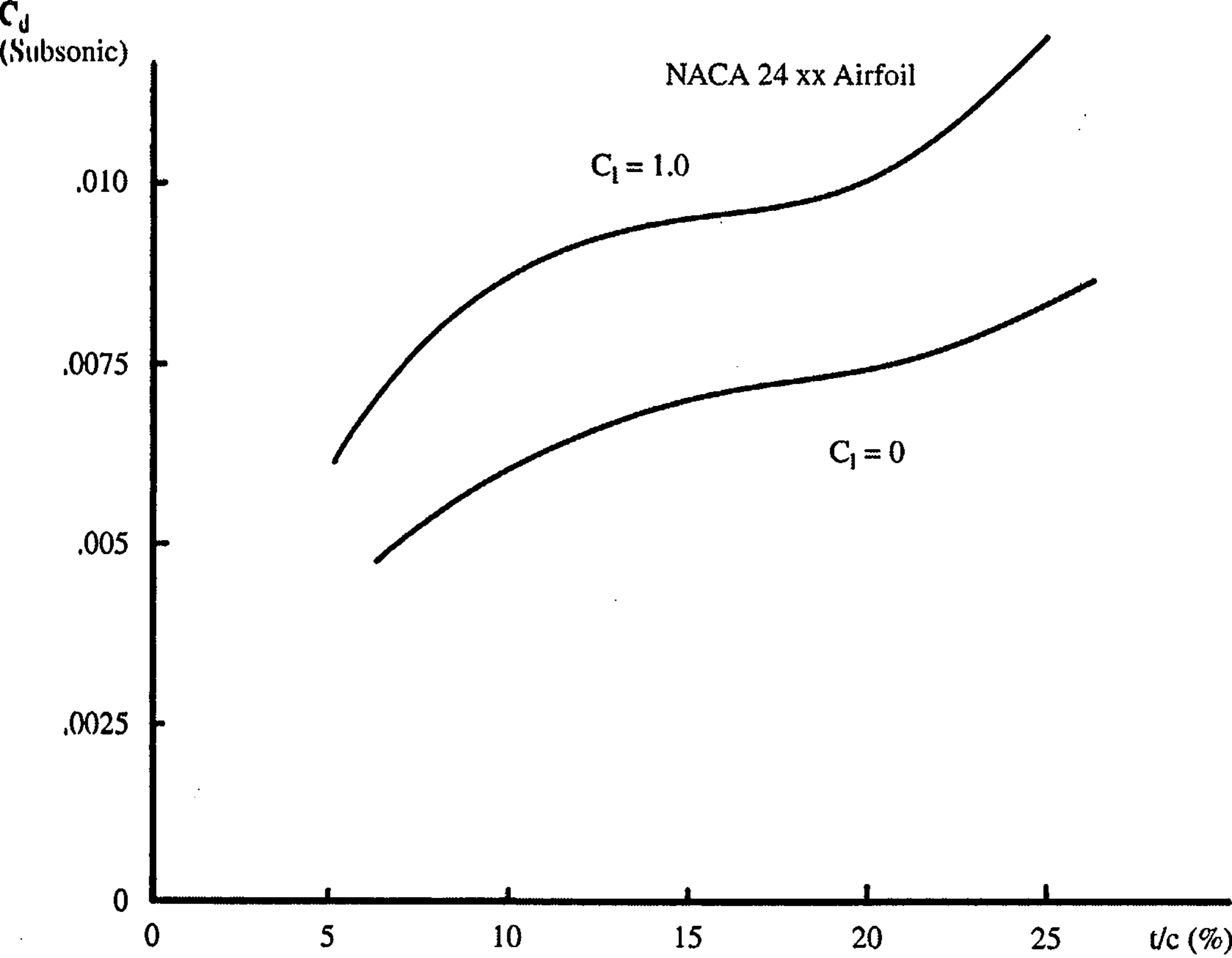
Fig. 4.11 Effect of t/c on drag.
