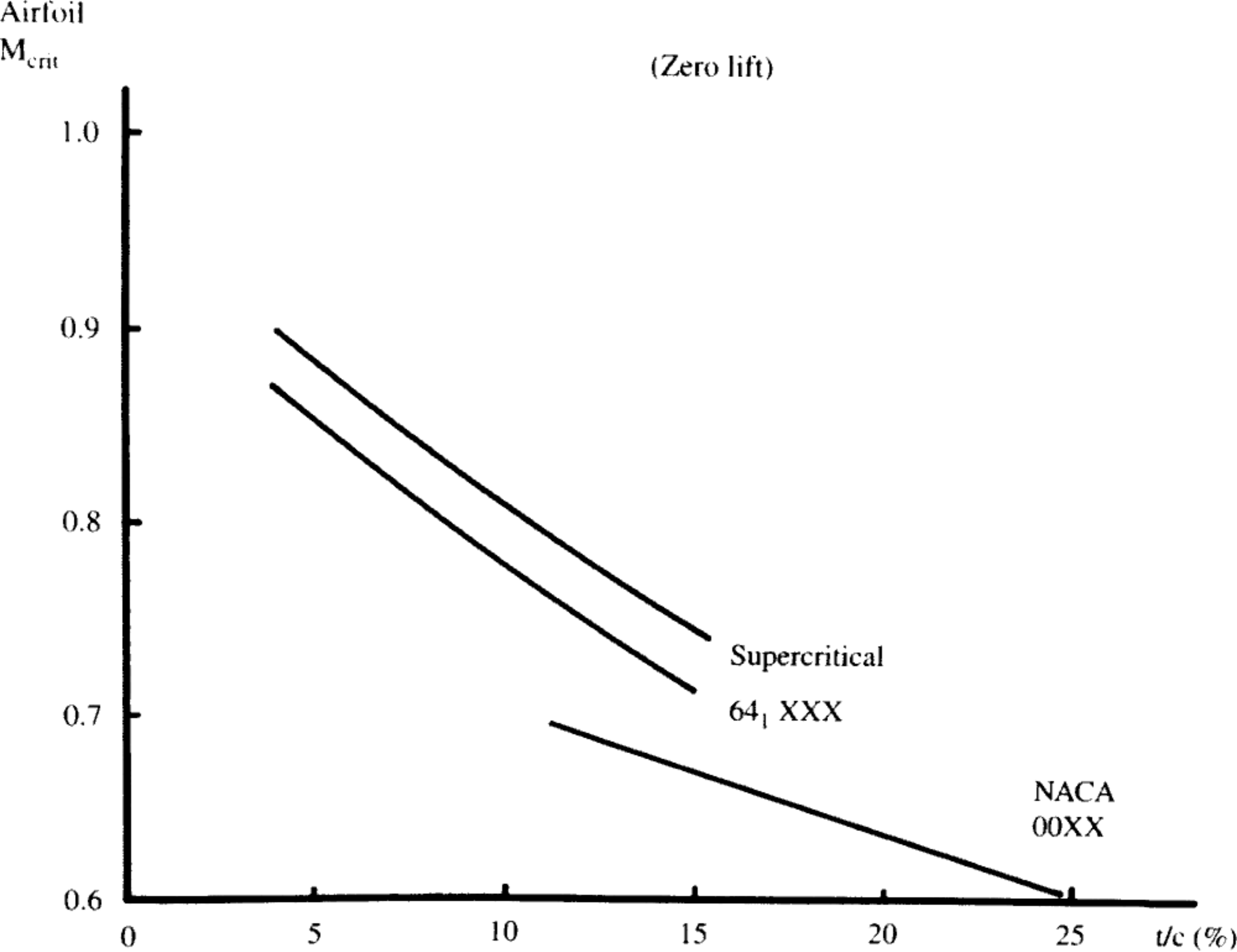
Fig. 4.12 Effect of t/c on critical Mach number.
