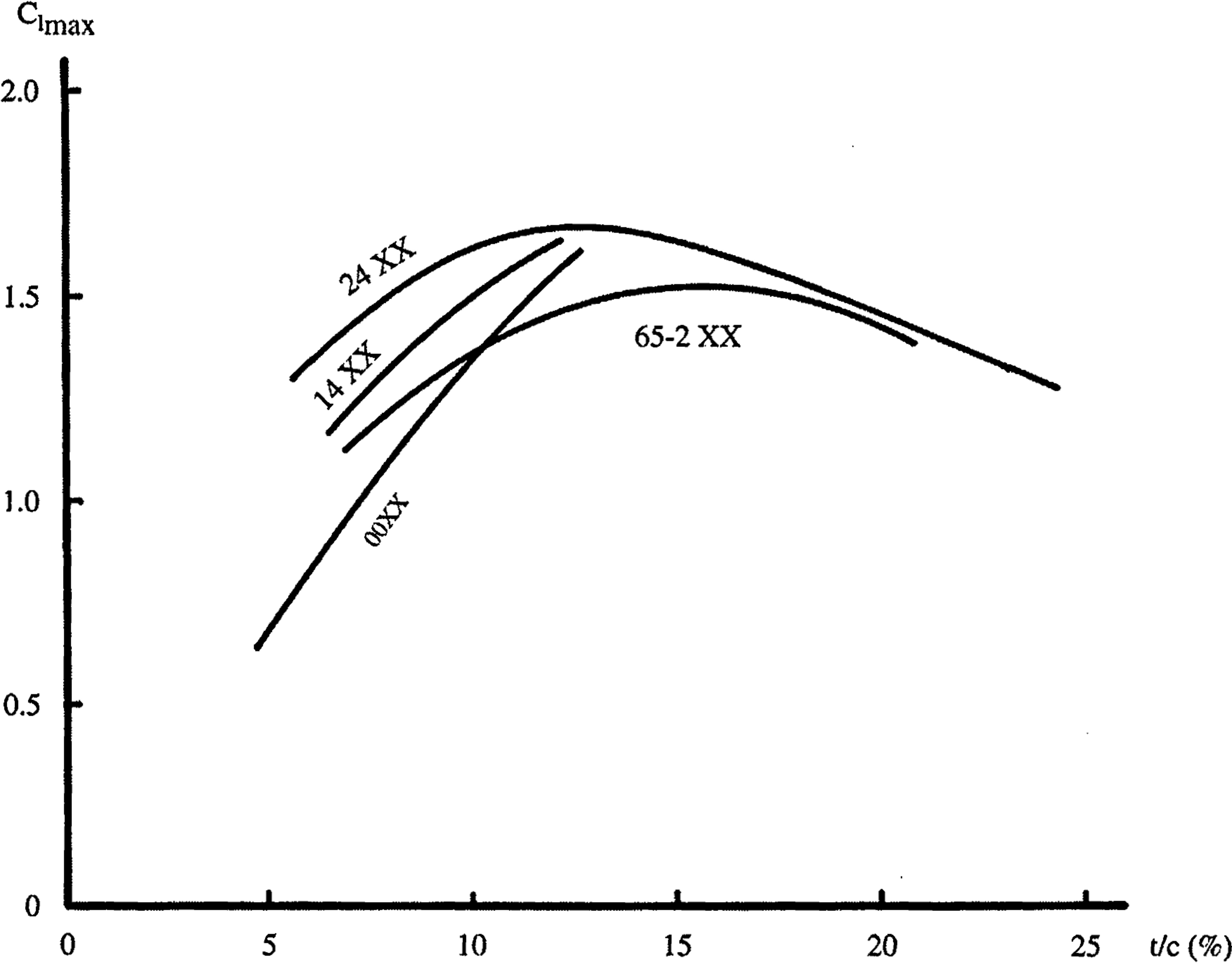
Fig. 4.13 Effect of t/c on maximum lift.
