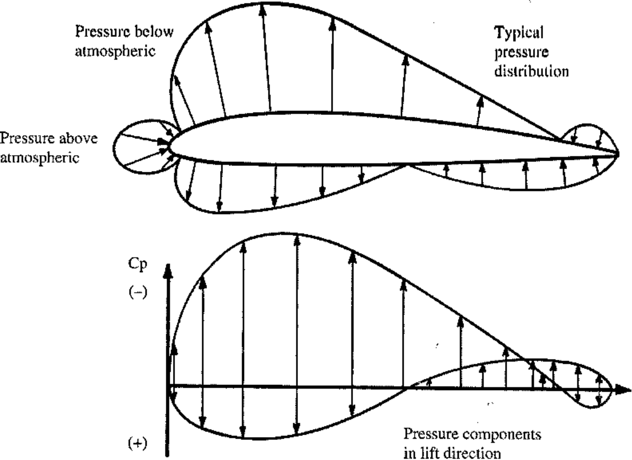
Fig. 4.2 Typical airfoil pressure distribution.
