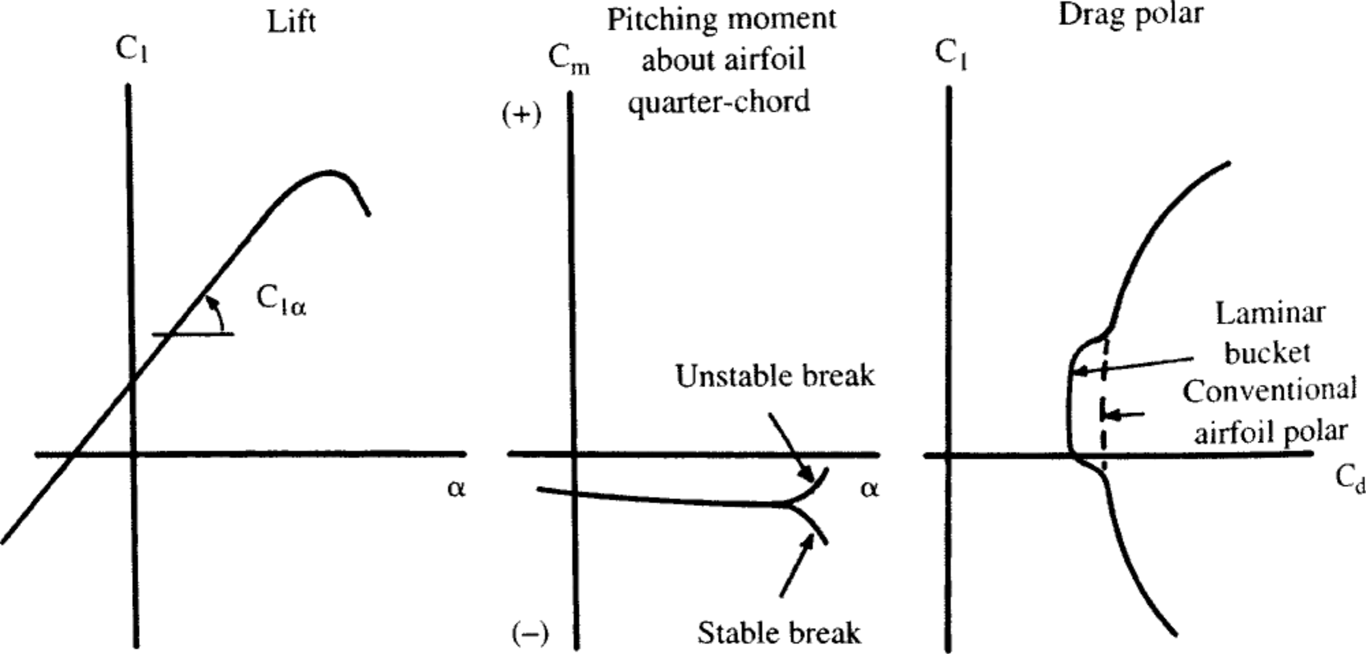
Fig. 4.5 Airfoil lift, drag, and pitching moment.
