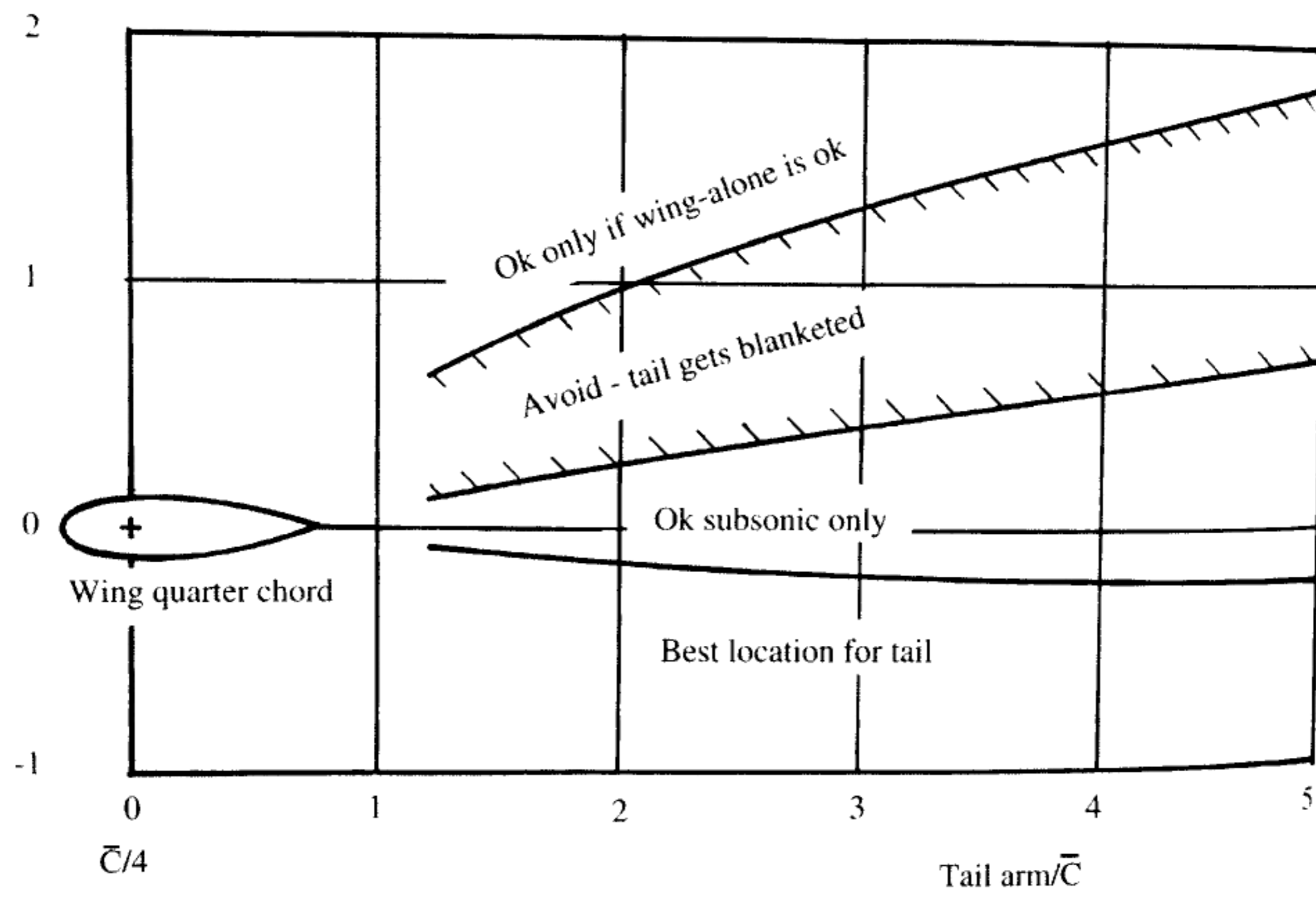
Fig. 4.33 Aft tail positioning.
